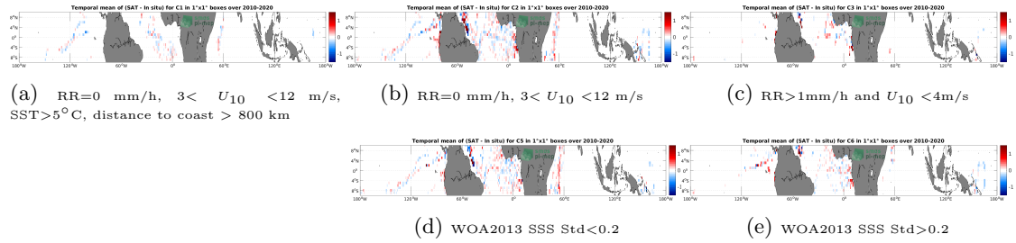
Figure 12: Temporal mean gridded over spatial boxes of size 1^{\circ}\times 1^{\circ} of \Delta SSS (SMOS SSS L3 v332 - 9 Days (CATDS-CPDC) - TSG (GOSUD-Research-vessel)) for 5 different subdatasets corresponding to:RR=0 mm/h, 3 < U_{10} < 12 m/s, SST >5^{\circ}\text{C} , distance to coast > 800 km (a), RR=0 mm/h, 3 < U_{10} < 12 m/s (b), RR >1 mm/h and U_{10} < 4 m/s (c), WOA2013 SSS Std <0.2 (d), WOA2013 SSS Std >0.2 (e).
