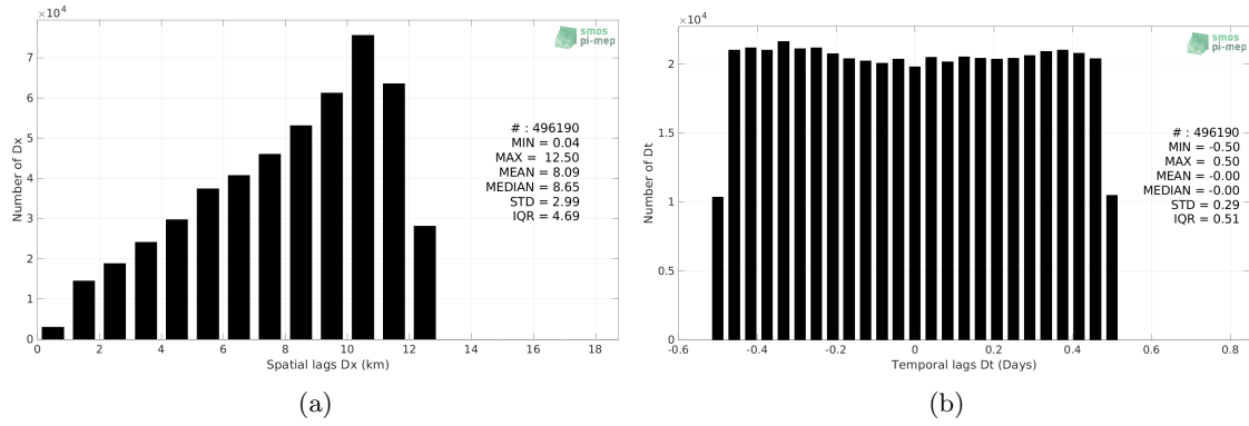
Figure 5: Histograms of the spatial (a) and temporal (b) lags between the location/time of the TSG (GOSUD-Research-vessel) measurement and the date of the corresponding SMOS SSS L3 v332 - 9 Days (CATDS-CPDC) SSS pixel.
