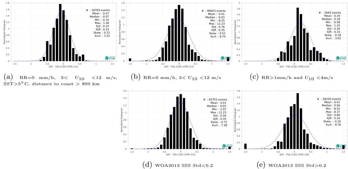
Figure 15: Normalized histogram of \Delta\text{SSS} (SMOS SSS L3 v332 - 9 Days (CATDS-CPDC) - TSG (CSIC-UTM)) for 5 different subdatasets corresponding to: RR=0 mm/h, 3 < U_{10} < 12 m/s, SST>5°C, distance to coast > 800 km (a), RR=0 mm/h, 3 < U_{10} < 12 m/s (b), RR>1mm/h and U_{10} < 4 m/s (c), WOA2013 SSS Std<0.2 (d), WOA2013 SSS Std>0.2 (e).
