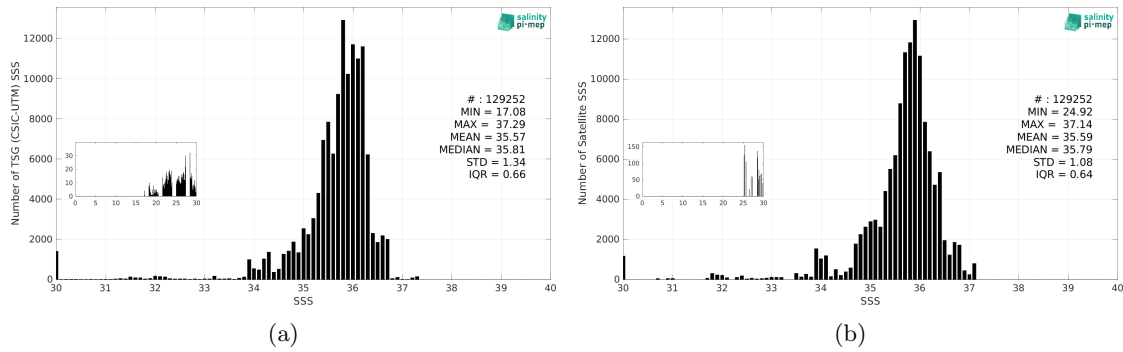
Figure 3: Histograms of SSS from TSG (CSIC-UTM) (a) and SMOS SSS L3 v332 - 9 Days (CATDS-CPDC) (b) considering all match-up pairs per bins of 0.1 over the Equatorial Ocean 10N-10S Pi-MEP region and for the full satellite product period.
