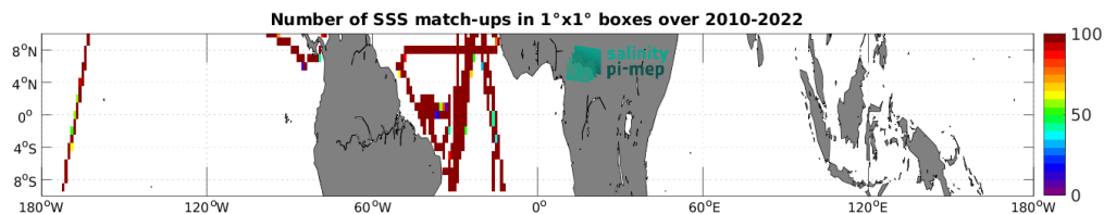
Figure 5: Number of SSS match-ups between TSG (CSIC-UTM) SSS and the SMOS SSS L3 v332 - 9 Days (CATDS-CPDC) SSS product for the Equatorial Ocean 10N-10S Pi-MEP region over 1^\circ \times 1^\circ boxes and for the full satellite product period.
