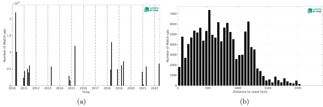
Figure 2: Number of match-ups between TSG (CSIC-UTM) and SMOS SSS L3 v332 - 9 Days (CATDS-CPDC) SSS as a function of time (a) and as function of the distance to coast (b) over the Equatorial Ocean 10N-10S Pi-MEP region and for the full satellite product period.
