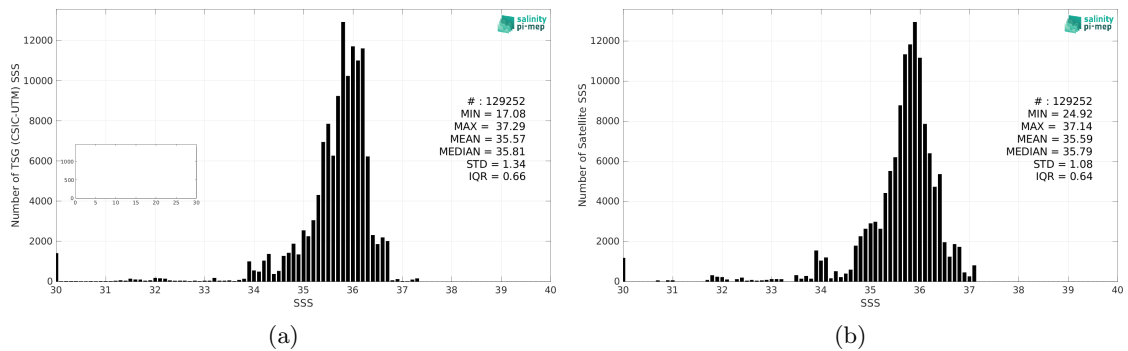
Figure 2: Histograms of SSS from TSG (CSIC-UTM) (a) and SMOS SSS L3 v332 - 9 Days (CATDS-CPDC) (b) considering all match-up pairs per bins of 0.1 over the Equatorial Ocean 10N-10S Pi-MEP region and for the full satellite product period.
