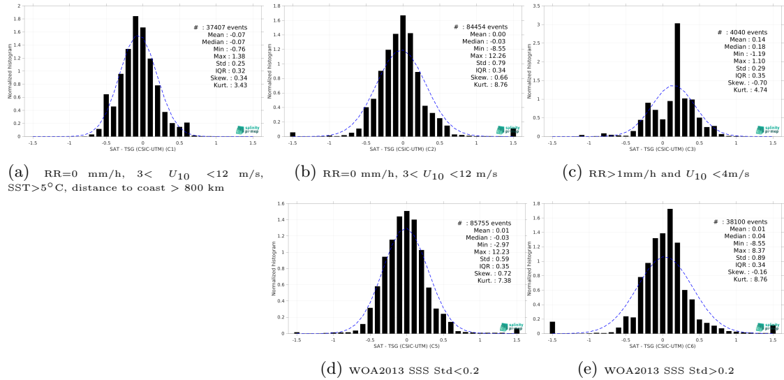
Figure 13: Normalized histogram of \Delta SSS (SMOS SSS L3 v332 - 9 Days (CATDS-CPDC) - TSG (CSIC-UTM)) for 5 different subdatasets corresponding to: RR=0 mm/h, 3 < U_{10} < 12 m/s, SST >5^\circ\text{C} , distance to coast > 800 km (a), RR=0 mm/h, 3 < U_{10} < 12 m/s (b), RR >1 mm/h and U_{10} < 4 m/s (c), WOA2013 SSS Std <0.2 (d), WOA2013 SSS Std >0.2 (e).
