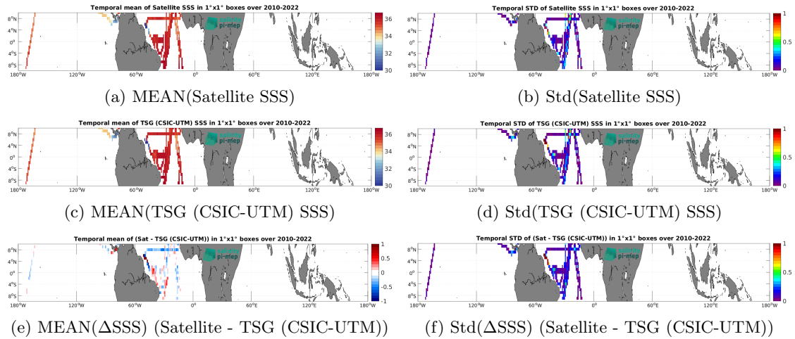
Figure 6: Temporal mean (left) and Std (right) of SSS from SMOS SSS L3 v332 - 9 Days (CATDS-CPDC) (top), TSG (CSIC-UTM) (middle), and of \Delta SSS (Satellite - TSG (CSIC-UTM)). Only match-up pairs are used to generate these maps.
