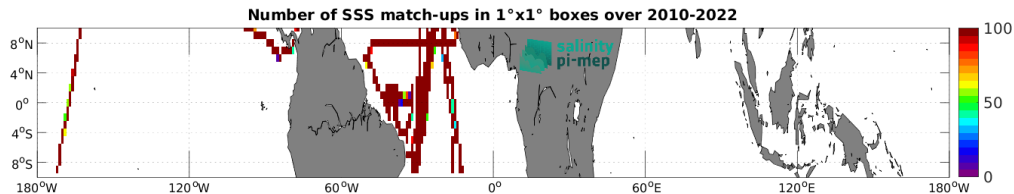
Figure 4: Number of SSS match-ups between TSG (CSIC-UTM) SSS and the SMOS SSS L3 v332 - 9 Days (CATDS-CPDC) SSS product for the Equatorial Ocean 10N-10S Pi-MEP region over 1^\circ \times 1^\circ boxes and for the full satellite product period.
