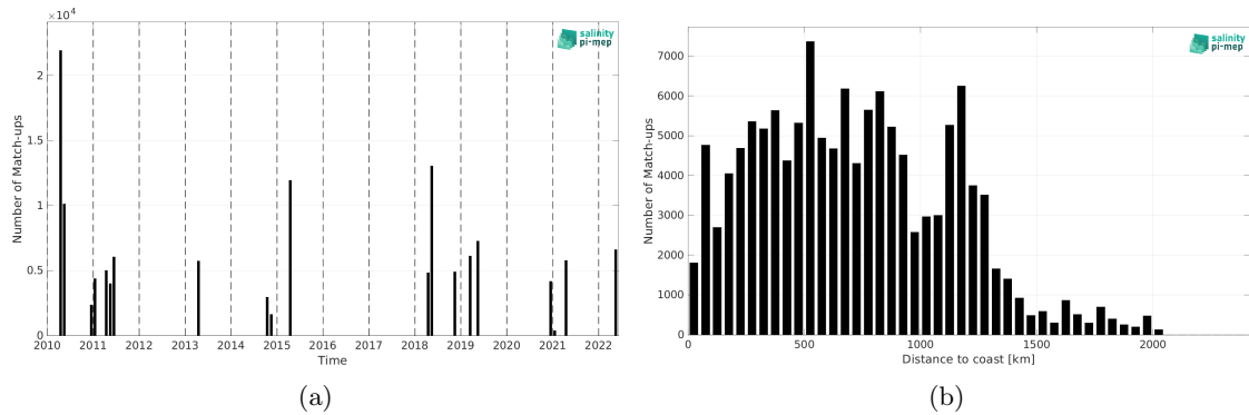
Figure 1: Number of match-ups between TSG (CSIC-UTM) and SMOS SSS L3 v332 - 9 Days (CATDS-CPDC) SSS as a function of time (a) and as function of the distance to coast (b) over the Equatorial Ocean 10N-10S Pi-MEP region and for the full satellite product period.
