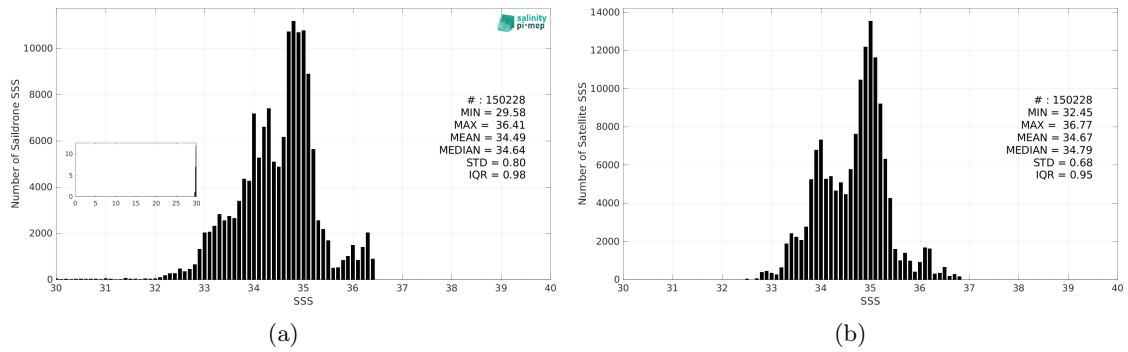
Figure 3: Histograms of SSS from Saildrone (a) and SMOS SSS L3 v332 - 9 Days (CATDS-CPDC) (b) considering all match-up pairs per bins of 0.1 over the Equatorial Ocean 10N-10S Pi-MEP region and for the full satellite product period.
