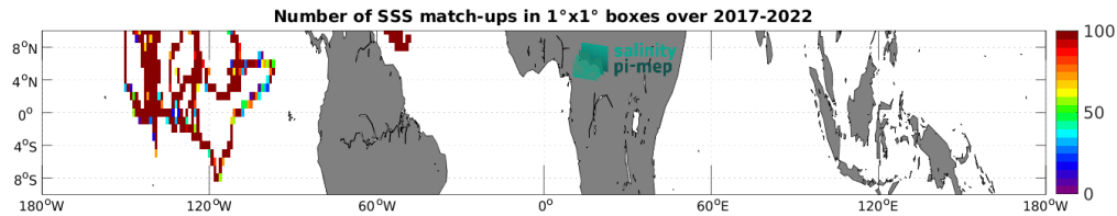
Figure 5: Number of SSS match-ups between Saildrone SSS and the SMOS SSS L3 v332 - 9 Days (CATDS-CPDC) SSS product for the Equatorial Ocean 10N-10S Pi-MEP region over 1^\circ \times 1^\circ boxes and for the full satellite product period.
