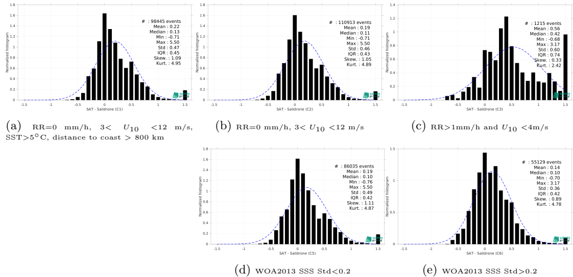
Figure 15: Normalized histogram of \Delta\text{SSS} (SMOS SSS L3 v332 - 9 Days (CATDS-CPDC) - Saildrone) for 5 different subdatasets corresponding to: RR=0 mm/h, 3 < U_{10} < 12 m/s, SST>5°C, distance to coast > 800 km (a), RR=0 mm/h, 3 < U_{10} < 12 m/s (b), RR>1mm/h and U_{10} < 4 m/s (c), WOA2013 SSS Std<0.2 (d), WOA2013 SSS Std>0.2 (e).
