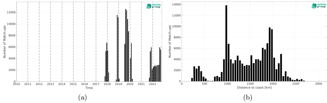
Figure 2: Number of match-ups between Saildrone and SMOS SSS L3 v332 - 9 Days (CATDS-CPDC) SSS as a function of time (a) and as function of the distance to coast (b) over the Equatorial Ocean 10N-10S Pi-MEP region and for the full satellite product period.
