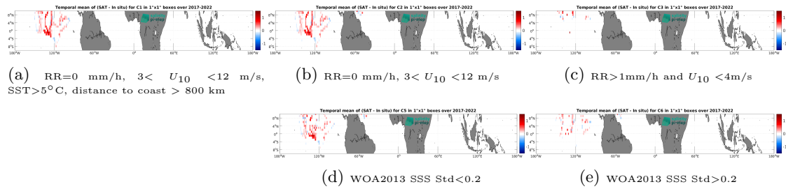
Figure 14: Temporal mean gridded over spatial boxes of size 1^\circ \times 1^\circ of \Delta\text{SSS} (SMOS SSS L3 v332 - 9 Days (CATDS-CPDC) - Saildrone) for 5 different subdatasets corresponding to: RR=0 mm/h, 3 < U_{10} < 12 m/s, SST>5°C, distance to coast > 800 km (a), RR=0 mm/h, 3 < U_{10} < 12 m/s (b), RR>1mm/h and U_{10} < 4 m/s (c), WOA2013 SSS Std<0.2 (d), WOA2013 SSS Std>0.2 (e).
