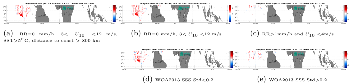
Figure 12: Temporal mean gridded over spatial boxes of size 1^\circ \times 1^\circ of \Delta SSS (SMOS SSS L3 v332 - 9 Days (CATDS-CPDC) - Saildrone) for 5 different subdatasets corresponding to: RR=0 mm/h, 3 < U_{10} < 12 m/s, SST >5^\circ C, distance to coast > 800 km (a), RR=0 mm/h, 3 < U_{10} < 12 m/s (b), RR >1 mm/h and U_{10} < 4 m/s (c), WOA2013 SSS Std <0.2 (d), WOA2013 SSS Std >0.2 (e).
