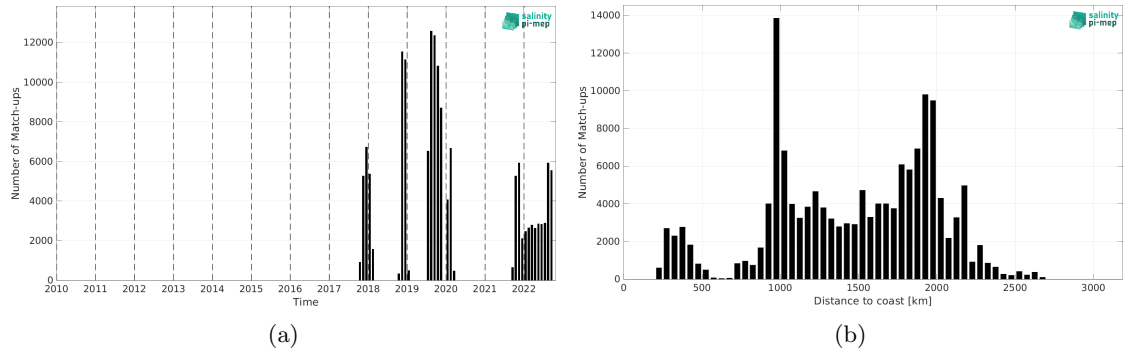
Figure 1: Number of match-ups between Saildrone and SMOS SSS L3 v332 - 9 Days (CATDS-CPDC) SSS as a function of time (a) and as function of the distance to coast (b) over the Equatorial Ocean 10N-10S Pi-MEP region and for the full satellite product period.
