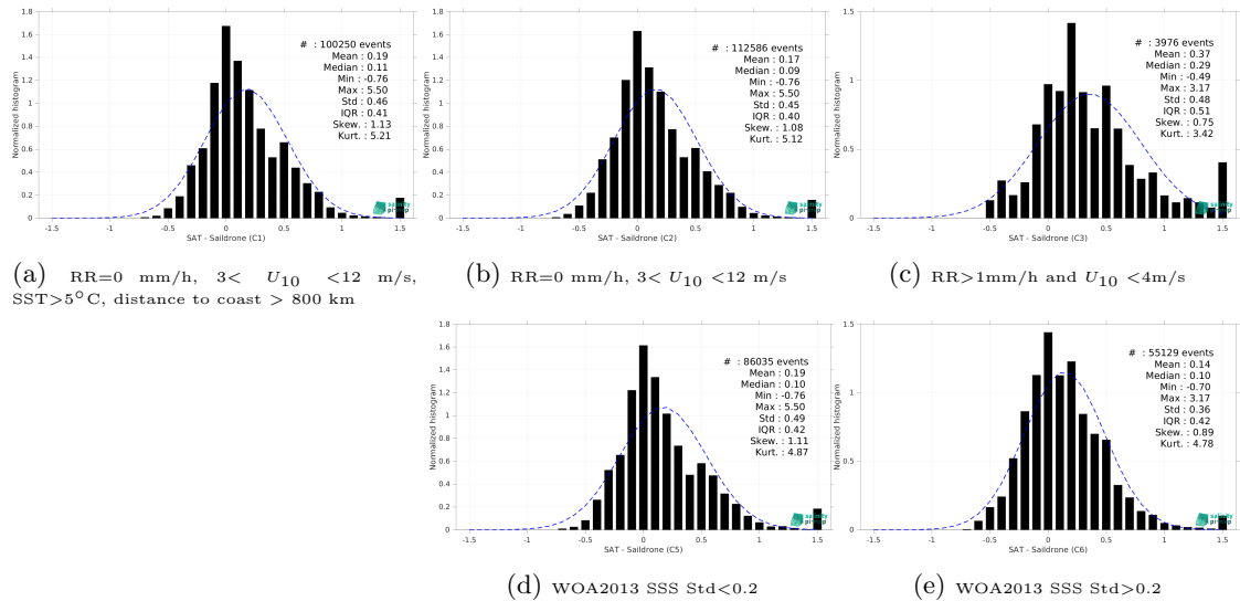
Figure 13: Normalized histogram of \Delta SSS (SMOS SSS L3 v332 - 9 Days (CATDS-CPDC) - Saildrone) for 5 different subdatasets corresponding to: RR=0 mm/h, 3 < U_{10} < 12 m/s, SST >5^\circ C, distance to coast > 800 km (a), RR=0 mm/h, 3 < U_{10} < 12 m/s (b), RR >1 mm/h and U_{10} < 4 m/s (c), WOA2013 SSS Std <0.2 (d), WOA2013 SSS Std >0.2 (e).
