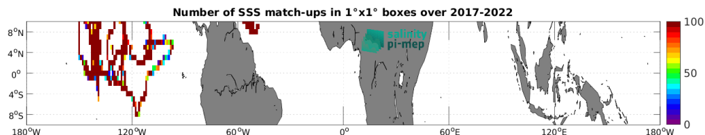
Figure 4: Number of SSS match-ups between Saildrone SSS and the SMOS SSS L3 v332 - 9 Days (CATDS-CPDC) SSS product for the Equatorial Ocean 10N-10S Pi-MEP region over 1^\circ \times 1^\circ boxes and for the full satellite product period.
