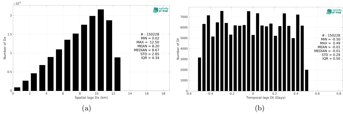
Figure 5: Histograms of the spatial (a) and temporal (b) lags between the location/time of the Sailability measurement and the date of the corresponding SMOS SSS L3 v332 - 9 Days (CATDS-CPDC) SSS pixel.
