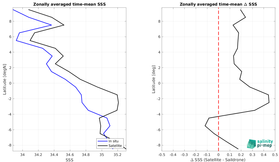
Figure 8: Left panel: Zonal mean SSS from SMOS SSS L3 v332 - 9 Days (CATDS-CPDC) satellite product (black) and from Sairdrone (blue). Right panel: Zonal mean of \Delta SSS (Satellite - Sairdrone) for all the collected Pi-MEP match-up pairs estimated over the full satellite product period.
