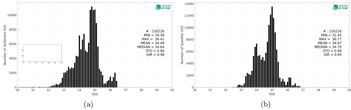
Figure 2: Histograms of SSS from Saildrone (a) and SMOS SSS L3 v332 - 9 Days (CATDS-CPDC) (b) considering all match-up pairs per bins of 0.1 over the Equatorial Ocean 10N-10S Pi-MEP region and for the full satellite product period.
