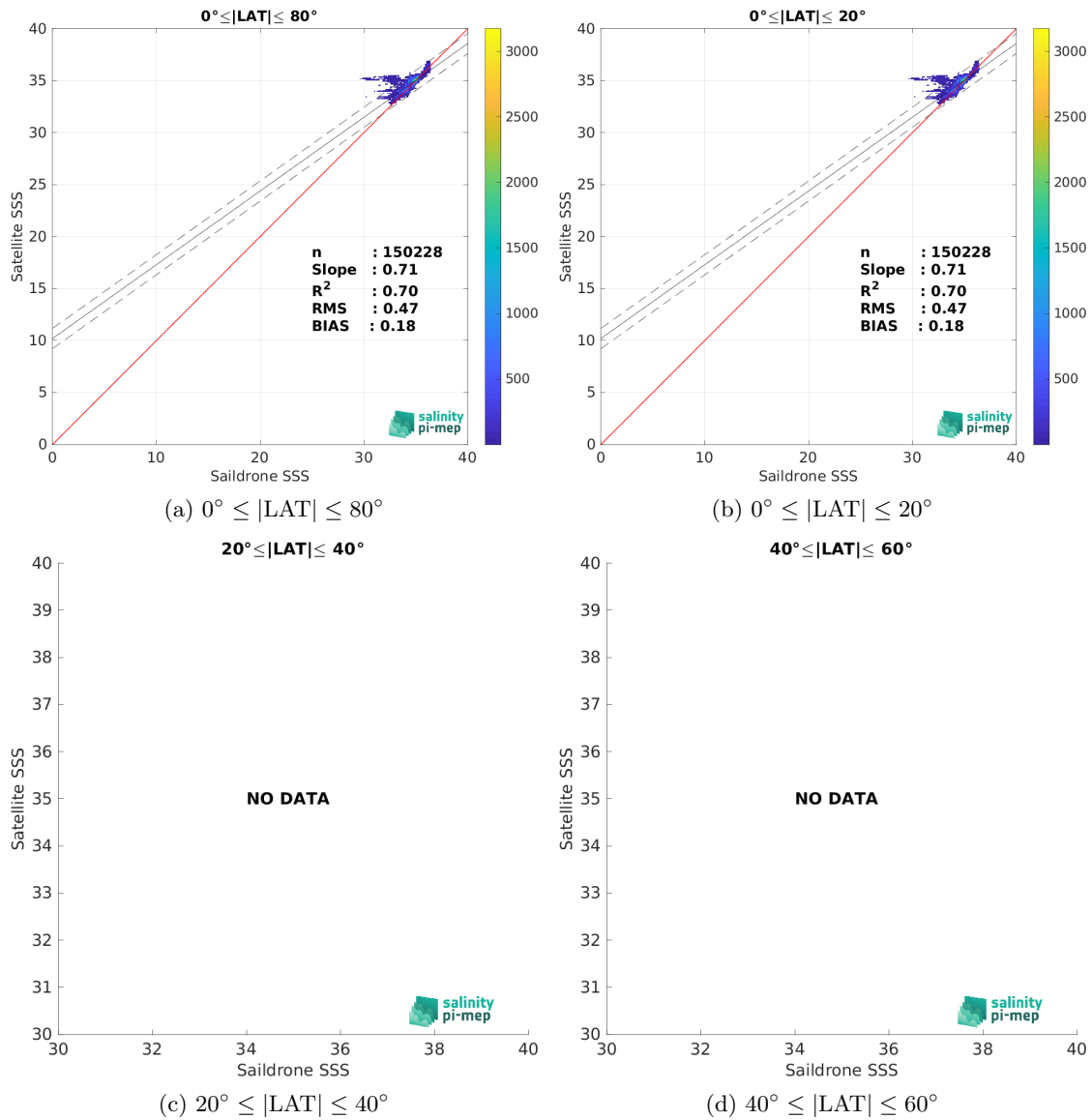
Figure 9: Contour maps of the concentration of SMOS SSS L3 v332 - 9 Days (CATDS-CPDC) SSS (y-axis) versus Sairdrone SSS (x-axis) at match-up pairs for different latitude bands. For each plot, the red line shows x=y . The black thin and dashed lines indicate a linear fit through the data cloud and the \pm 95\% confidence levels, respectively. The number match-up pairs n , the slope and R^2 coefficient of the linear fit, the root mean square (RMS) and the mean bias between satellite and in situ data are indicated for each latitude band in each plots.
