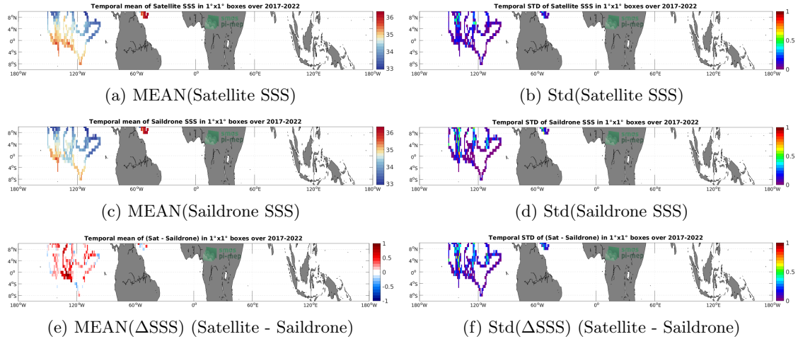
Figure 6: Temporal mean (left) and Std (right) of SSS from SMOS SSS L3 v332 - 9 Days (CATDS-CPDC) (top), Sairdrone (middle), and of \Delta SSS (Satellite - Sairdrone). Only match-up pairs are used to generate these maps.
