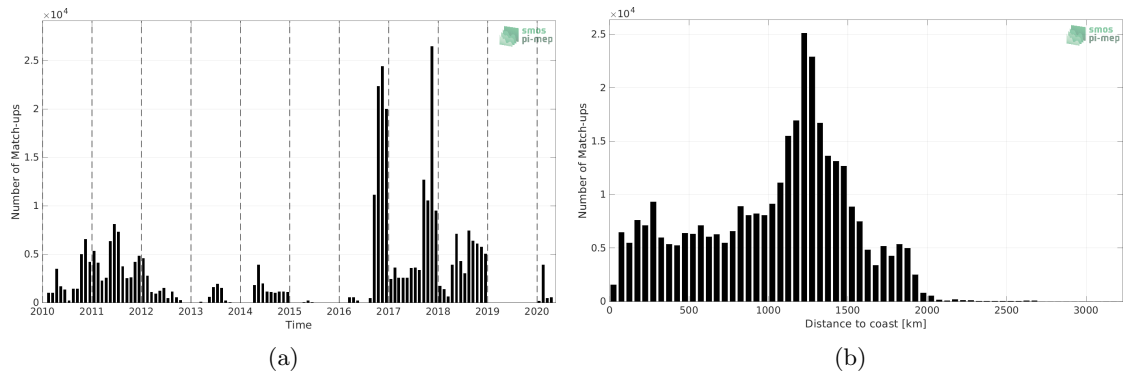
Figure 1: Number of match-ups between Surface drifters and SMOS SSS L3 v332 - 9 Days (CATDS-CPDC) SSS as a function of time (a) and as function of the distance to coast (b) over the Equatorial Ocean 10N-10S Pi-MEP region and for the full satellite product period.
