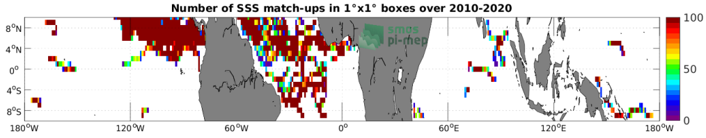
Figure 3: Number of SSS match-ups between Surface drifters SSS and the SMOS SSS L3 v332 - 9 Days (CATDS-CPDC) SSS product for the Equatorial Ocean 10N-10S Pi-MEP region over 1^\circ \times 1^\circ boxes and for the full satellite product period.
