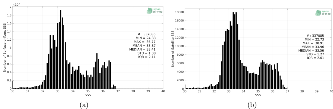
Figure 2: Histograms of SSS from Surface drifters (a) and SMOS SSS L3 v332 - 9 Days (CATDS-CPDC) (b) considering all match-up pairs per bins of 0.1 over the Equatorial Ocean 10N-10S Pi-MEP region and for the full satellite product period.
