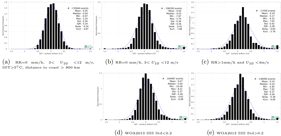
Figure 12: Normalized histogram of \Delta SSS (SMOS SSS L3 v332 - 9 Days (CATDS-CPDC) - Surface drifters) for 5 different subdatasets corresponding to: RR=0 mm/h, 3 < U_{10} < 12 m/s, SST >5^\circ\text{C} , distance to coast > 800 km (a), RR=0 mm/h, 3 < U_{10} < 12 m/s (b), RR >1 mm/h and U_{10} < 4 m/s (c), WOA2013 SSS Std <0.2 (d), WOA2013 SSS Std >0.2 (e).
