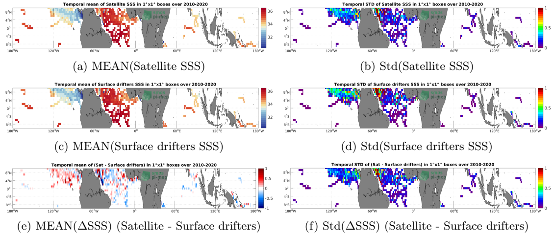
Figure 5: Temporal mean (left) and Std (right) of SSS from SMOS SSS L3 v332 - 9 Days (CATDS-CPDC) (top), Surface drifters (middle), and of \Delta SSS (Satellite - Surface drifters). Only match-up pairs are used to generate these maps.
