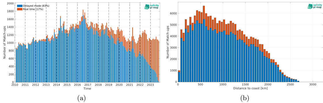
Figure 1: Number of match-ups between Argo and SMOS SSS L3 v332 - 9 Days (CATDS-CPDC) SSS as a function of time (a) and as function of the distance to coast (b) over the Equatorial Ocean 10N-10S Pi-MEP region and for the full satellite product period.
