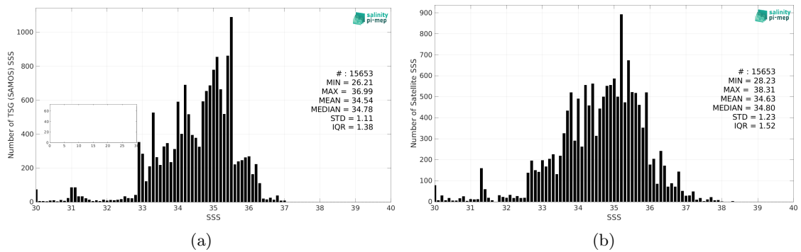
Figure 2: Histograms of SSS from TSG (SAMOS) (a) and SMOS SSS L2Q v331 - 0.25 Deg (CATDS-CPDC) (b) considering all match-up pairs per bins of 0.1 over the Equatorial Ocean 10N-10S Pi-MEP region and for the full satellite product period.
