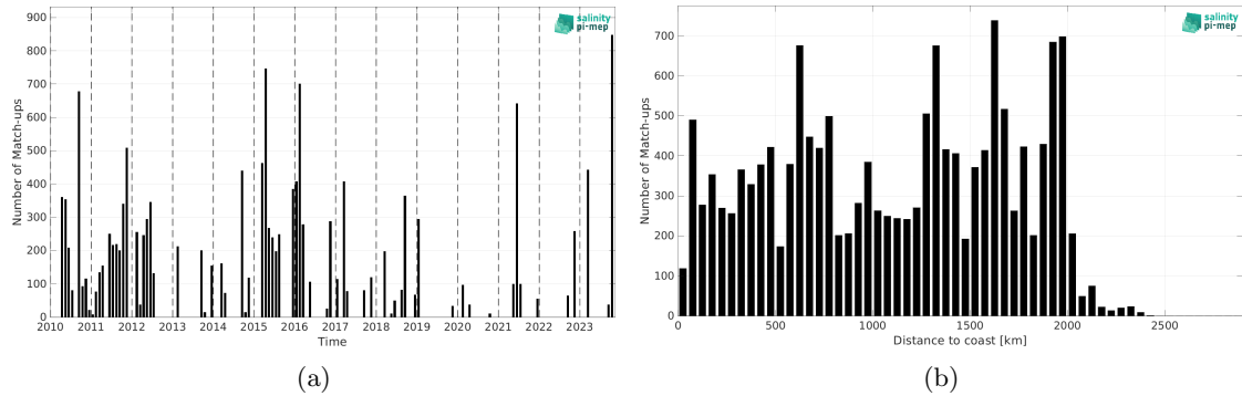
Figure 1: Number of match-ups between TSG (SAMOS) and SMOS SSS L2Q v331 - 0.25 Deg (CATDS-CPDC) SSS as a function of time (a) and as function of the distance to coast (b) over the Equatorial Ocean 10N-10S Pi-MEP region and for the full satellite product period.
