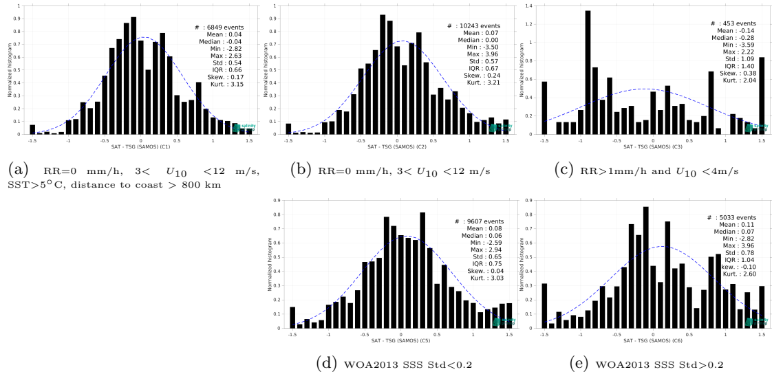
Figure 13: Normalized histogram of \Delta SSS (SMOS SSS L2Q v331 - 0.25 Deg (CATDS-CPDC) - TSG (SAMOS)) for 5 different subdatasets corresponding to: RR=0 mm/h, 3 < U_{10} < 12 m/s, SST >5^\circ C, distance to coast > 800 km (a), RR=0 mm/h, 3 < U_{10} < 12 m/s (b), RR >1 mm/h and U_{10} < 4 m/s (c), WOA2013 SSS Std <0.2 (d), WOA2013 SSS Std >0.2 (e).
