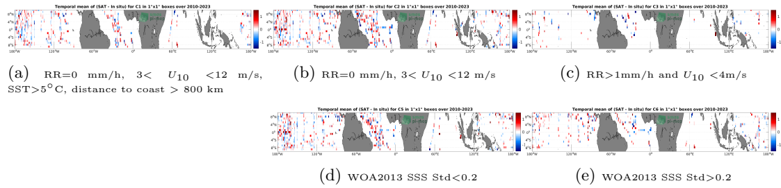
Figure 12: Temporal mean gridded over spatial boxes of size 1^\circ \times 1^\circ of \Delta SSS (SMOS SSS L2Q v331 - 0.25 Deg (CATDS-CPDC) - TSG (SAMOS)) for 5 different subdatasets corresponding to: RR=0 mm/h, 3 < U_{10} < 12 m/s, SST>5°C, distance to coast > 800 km (a), RR=0 mm/h, 3 < U_{10} < 12 m/s (b), RR>1mm/h and U_{10} < 4 m/s (c), WOA2013 SSS Std<0.2 (d), WOA2013 SSS Std>0.2 (e).
