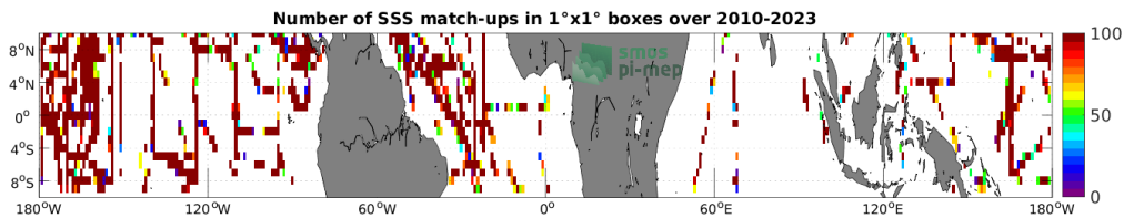
Figure 4: Number of SSS match-ups between TSG (SAMOS) SSS and the SMOS SSS L2Q v331 - 0.25 Deg (CATDS-CPDC) SSS product for the Equatorial Ocean 10N-10S Pi-MEP region over 1^\circ \times 1^\circ boxes and for the full satellite product period.
