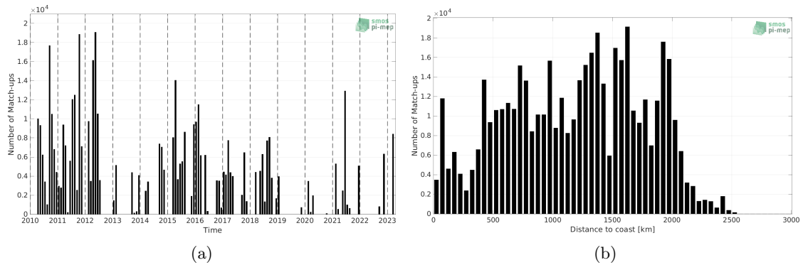
Figure 1: Number of match-ups between TSG (SAMOS) and SMOS SSS L2Q v331 - 0.25 Deg (CATDS-CPDC) SSS as a function of time (a) and as function of the distance to coast (b) over the Equatorial Ocean 10N-10S Pi-MEP region and for the full satellite product period.
