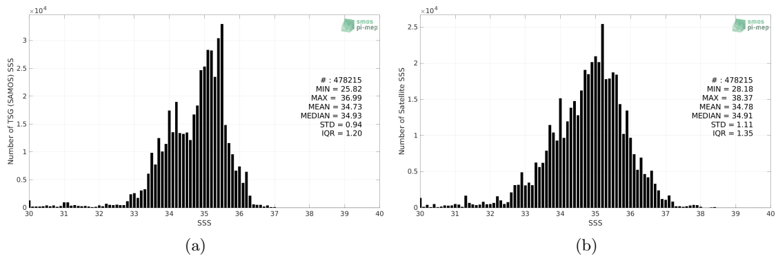
Figure 2: Histograms of SSS from TSG (SAMOS) (a) and SMOS SSS L2Q v331 - 0.25 Deg (CATDS-CPDC) (b) considering all match-up pairs per bins of 0.1 over the Equatorial Ocean 10N-10S Pi-MEP region and for the full satellite product period.
