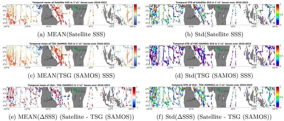
Figure 6: Temporal mean (left) and Std (right) of SSS from SMOS SSS L2Q v331 - 0.25 Deg (CATDS-CPDC) (top), TSG (SAMOS) (middle), and of \Delta SSS (Satellite - TSG (SAMOS)). Only match-up pairs are used to generate these maps.
