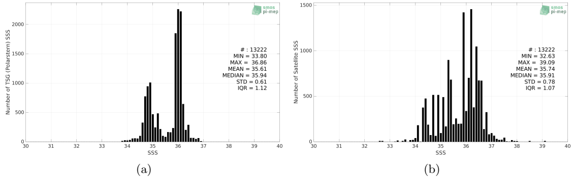
Figure 2: Histograms of SSS from TSG (Polarstern) (a) and SMOS SSS L2Q v331 - 0.25 Deg (CATDS-CPDC) (b) considering all match-up pairs per bins of 0.1 over the Equatorial Ocean 10N-10S Pi-MEP region and for the full satellite product period.
