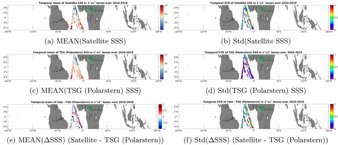
Figure 6: Temporal mean (left) and Std (right) of SSS from SMOS SSS L2Q v331 - 0.25 Deg (CATDS-CPDC) (top), TSG (Polarstern) (middle), and of \Delta SSS (Satellite - TSG (Polarstern)). Only match-up pairs are used to generate these maps.
