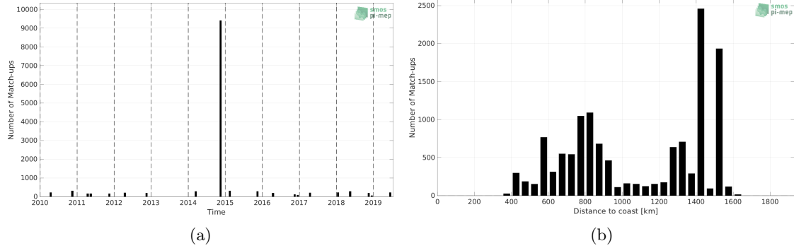
Figure 1: Number of match-ups between TSG (Polarstern) and SMOS SSS L2Q v331 - 0.25 Deg (CATDS-CPDC) SSS as a function of time (a) and as function of the distance to coast (b) over the Equatorial Ocean 10N-10S Pi-MEP region and for the full satellite product period.
