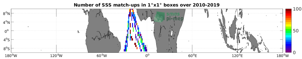
Figure 4: Number of SSS match-ups between TSG (Polarstern) SSS and the SMOS SSS L2Q v331 - 0.25 Deg (CATDS-CPDC) SSS product for the Equatorial Ocean 10N-10S Pi-MEP region over 1^\circ \times 1^\circ boxes and for the full satellite product period.
