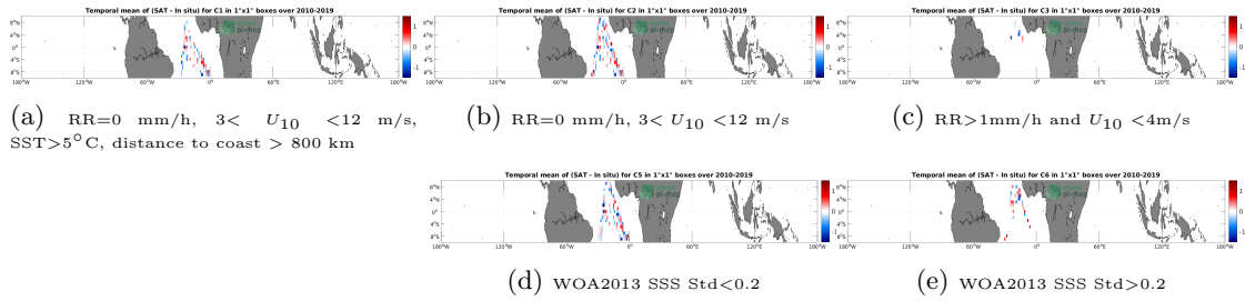
Figure 12: Temporal mean gridded over spatial boxes of size 1^\circ \times 1^\circ of \Delta SSS (SMOS SSS L2Q v331 - 0.25 Deg (CATDS-CPDC) - TSG (Polarstern)) for 5 different subdatasets corresponding to: RR=0 mm/h, 3 < U_{10} < 12 m/s, SST>5°C, distance to coast > 800 km (a), RR=0 mm/h, 3 < U_{10} < 12 m/s (b), RR>1mm/h and U_{10} < 4 m/s (c), WOA2013 SSS Std<0.2 (d), WOA2013 SSS Std>0.2 (e).
