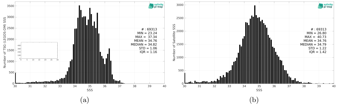
Figure 2: Histograms of SSS from TSG (LEGOS-DM) (a) and SMOS SSS L2Q v331 - 0.25 Deg (CATDS-CPDC) (b) considering all match-up pairs per bins of 0.1 over the Equatorial Ocean 10N-10S Pi-MEP region and for the full satellite product period.
