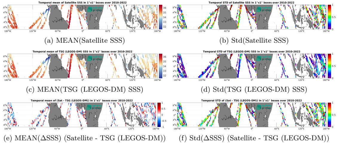
Figure 6: Temporal mean (left) and Std (right) of SSS from SMOS SSS L2Q v331 - 0.25 Deg (CATDS-CPDC) (top), TSG (LEGOS-DM) (middle), and of \Delta SSS (Satellite - TSG (LEGOS-DM)). Only match-up pairs are used to generate these maps.
