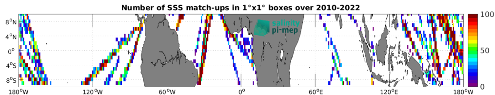
Figure 4: Number of SSS match-ups between TSG (LEGOS-DM) SSS and the SMOS SSS L2Q v331 - 0.25 Deg (CATDS-CPDC) SSS product for the Equatorial Ocean 10N-10S Pi-MEP region over 1^\circ \times 1^\circ boxes and for the full satellite product period.
