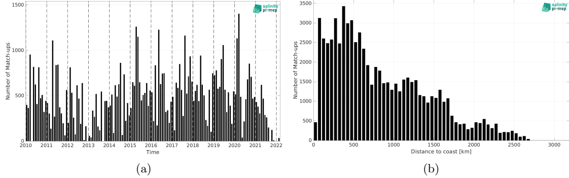
Figure 1: Number of match-ups between TSG (LEGOS-DM) and SMOS SSS L2Q v331 - 0.25 Deg (CATDS-CPDC) SSS as a function of time (a) and as function of the distance to coast (b) over the Equatorial Ocean 10N-10S Pi-MEP region and for the full satellite product period.
