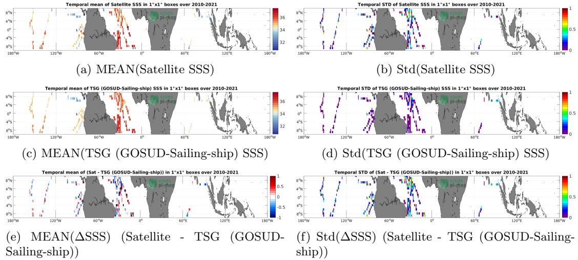
Figure 6: Temporal mean (left) and Std (right) of SSS from SMOS SSS L2Q v331 - 0.25 Deg (CATDS-CPDC) (top), TSG (GOSUD-Sailing-ship) (middle), and of \Delta SSS (Satellite - TSG (GOSUD-Sailing-ship)). Only match-up pairs are used to generate these maps.
