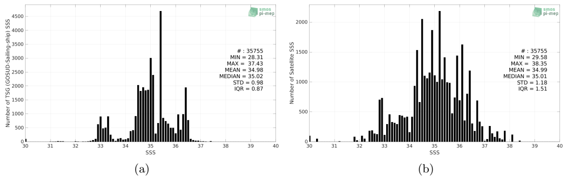
Figure 2: Histograms of SSS from TSG (GOSUD-Sailing-ship) (a) and SMOS SSS L2Q v331 - 0.25 Deg (CATDS-CPDC) (b) considering all match-up pairs per bins of 0.1 over the Equatorial Ocean 10N-10S Pi-MEP region and for the full satellite product period.
