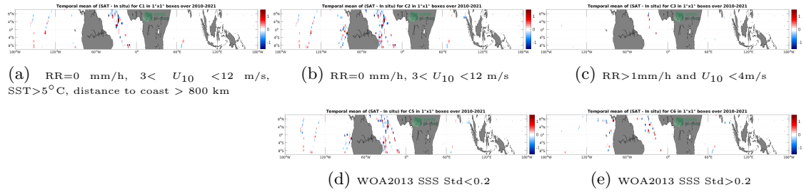
Figure 12: Temporal mean gridded over spatial boxes of size 1^\circ \times 1^\circ of \Delta SSS (SMOS SSS L2Q v331 - 0.25 Deg (CATDS-CPDC) - TSG (GOSUD-Sailing-ship)) for 5 different subdatasets corresponding to:RR=0 mm/h, 3 < U_{10} < 12 m/s, SST >5^\circ\text{C} , distance to coast > 800 km (a), RR=0 mm/h, 3 < U_{10} < 12 m/s (b), RR >1 mm/h and U_{10} < 4 m/s (c), WOA2013 SSS Std <0.2 (d), WOA2013 SSS Std >0.2 (e).
