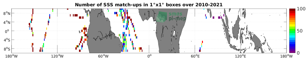
Figure 4: Number of SSS match-ups between TSG (GOSUD-Sailing-ship) SSS and the SMOS SSS L2Q v331 - 0.25 Deg (CATDS-CPDC) SSS product for the Equatorial Ocean 10N-10S Pi-MEP region over 1^\circ \times 1^\circ boxes and for the full satellite product period.
