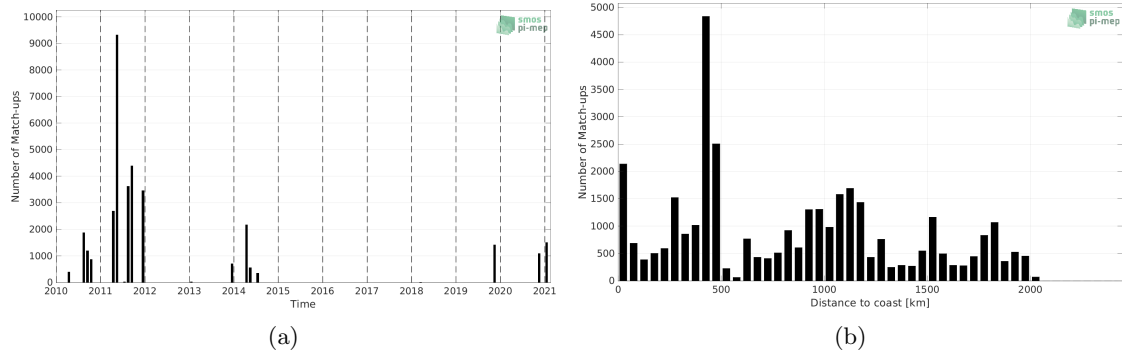
Figure 1: Number of match-ups between TSG (GOSUD-Sailing-ship) and SMOS SSS L2Q v331 - 0.25 Deg (CATDS-CPDC) SSS as a function of time (a) and as function of the distance to coast (b) over the Equatorial Ocean 10N-10S Pi-MEP region and for the full satellite product period.
