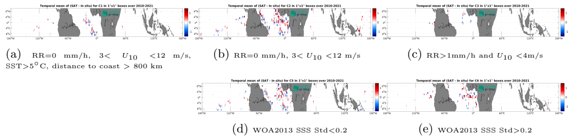
Figure 12: Temporal mean gridded over spatial boxes of size 1^{\circ}\times 1^{\circ} of \Delta SSS (SMOS SSS L2Q v331 - 0.25 Deg (CATDS-CPDC) - TSG (GOSUD-Research-vessel)) for 5 different subdatasets corresponding to:RR=0 mm/h, 3 < U_{10} < 12 m/s, SST >5^{\circ}\text{C} , distance to coast > 800 km (a), RR=0 mm/h, 3 < U_{10} < 12 m/s (b), RR >1 mm/h and U_{10} < 4 m/s (c), WOA2013 SSS Std <0.2 (d), WOA2013 SSS Std >0.2 (e).
