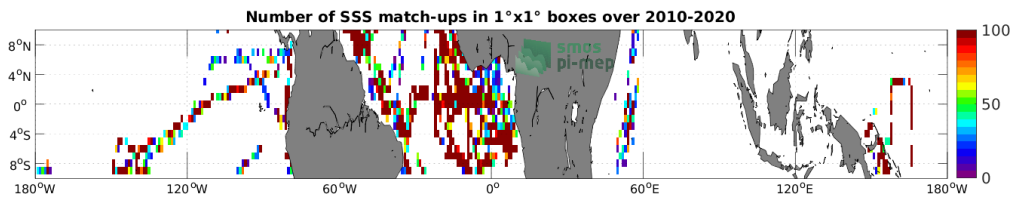
Figure 4: Number of SSS match-ups between TSG (GOSUD-Research-vessel) SSS and the SMOS SSS L2Q v331 - 0.25 Deg (CATDS-CPDC) SSS product for the Equatorial Ocean 10N-10S Pi-MEP region over 1^\circ \times 1^\circ boxes and for the full satellite product period.
