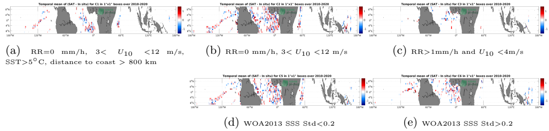
Figure 12: Temporal mean gridded over spatial boxes of size 1^{\circ}\times 1^{\circ} of \Delta SSS (SMOS SSS L2Q v331 - 0.25 Deg (CATDS-CPDC) - TSG (GOSUD-Research-vessel)) for 5 different subdatasets corresponding to:RR=0 mm/h, 3 < U_{10} < 12 m/s, SST >5^{\circ}\text{C} , distance to coast > 800 km (a), RR=0 mm/h, 3 < U_{10} < 12 m/s (b), RR >1 mm/h and U_{10} < 4 m/s (c), WOA2013 SSS Std <0.2 (d), WOA2013 SSS Std >0.2 (e).
