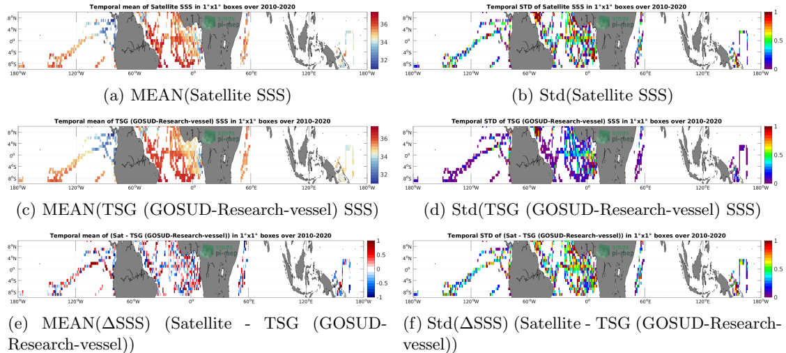
Figure 6: Temporal mean (left) and Std (right) of SSS from SMOS SSS L2Q v331 - 0.25 Deg (CATDS-CPDC) (top), TSG (GOSUD-Research-vessel) (middle), and of \Delta SSS (Satellite - TSG (GOSUD-Research-vessel)). Only match-up pairs are used to generate these maps.
