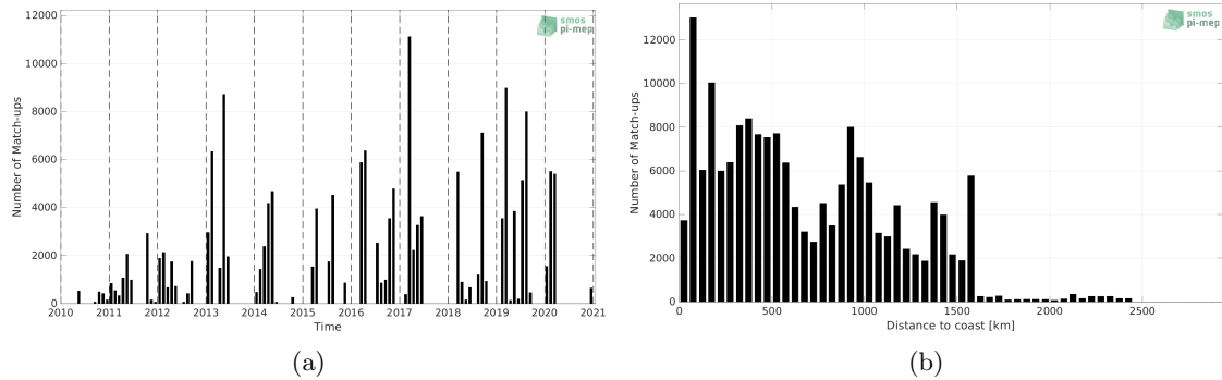
Figure 1: Number of match-ups between TSG (GOSUD-Research-vessel) and SMOS SSS L2Q v331 - 0.25 Deg (CATDS-CPDC) SSS as a function of time (a) and as function of the distance to coast (b) over the Equatorial Ocean 10N-10S Pi-MEP region and for the full satellite product period.
