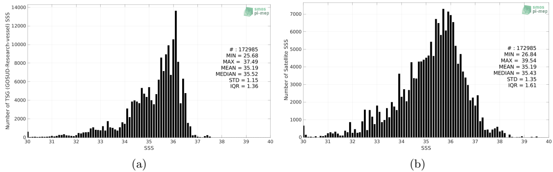
Figure 2: Histograms of SSS from TSG (GOSUD-Research-vessel) (a) and SMOS SSS L2Q v331 - 0.25 Deg (CATDS-CPDC) (b) considering all match-up pairs per bins of 0.1 over the Equatorial Ocean 10N-10S Pi-MEP region and for the full satellite product period.
