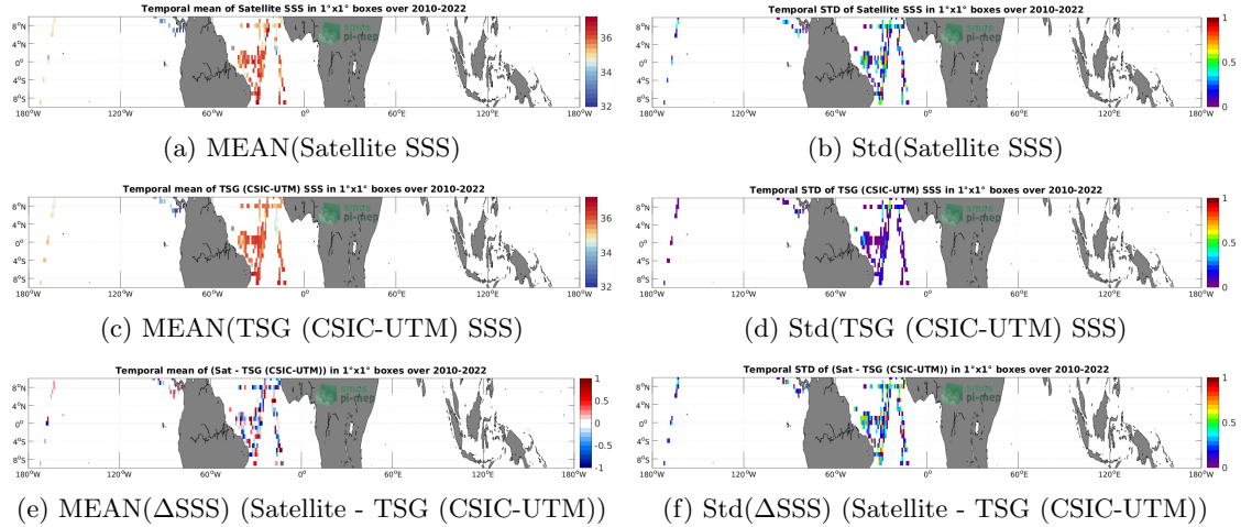
Figure 6: Temporal mean (left) and Std (right) of SSS from SMOS SSS L2Q v331 - 0.25 Deg (CATDS-CPDC) (top), TSG (CSIC-UTM) (middle), and of \Delta SSS (Satellite - TSG (CSIC-UTM)). Only match-up pairs are used to generate these maps.
