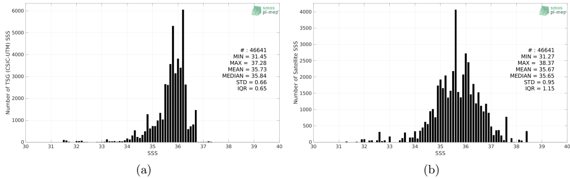
Figure 2: Histograms of SSS from TSG (CSIC-UTM) (a) and SMOS SSS L2Q v331 - 0.25 Deg (CATDS-CPDC) (b) considering all match-up pairs per bins of 0.1 over the Equatorial Ocean 10N-10S Pi-MEP region and for the full satellite product period.
