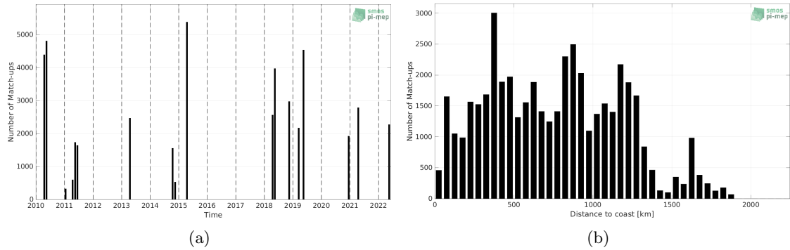
Figure 1: Number of match-ups between TSG (CSIC-UTM) and SMOS SSS L2Q v331 - 0.25 Deg (CATDS-CPDC) SSS as a function of time (a) and as function of the distance to coast (b) over the Equatorial Ocean 10N-10S Pi-MEP region and for the full satellite product period.
