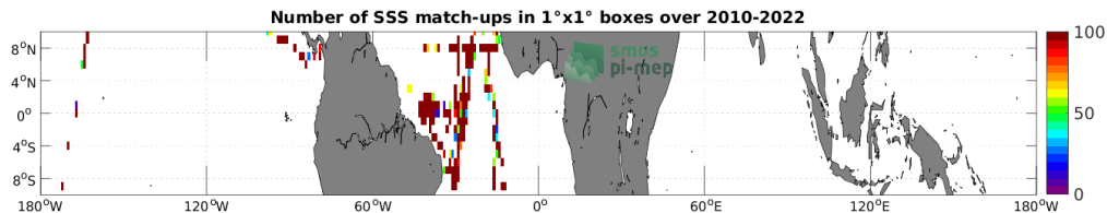
Figure 4: Number of SSS match-ups between TSG (CSIC-UTM) SSS and the SMOS SSS L2Q v331 - 0.25 Deg (CATDS-CPDC) SSS product for the Equatorial Ocean 10N-10S Pi-MEP region over 1^\circ \times 1^\circ boxes and for the full satellite product period.
