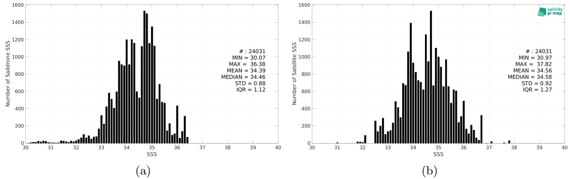
Figure 2: Histograms of SSS from Saildrone (a) and SMOS SSS L2Q v331 - 0.25 Deg (CATDS-CPDC) (b) considering all match-up pairs per bins of 0.1 over the Equatorial Ocean 10N-10S Pi-MEP region and for the full satellite product period.
