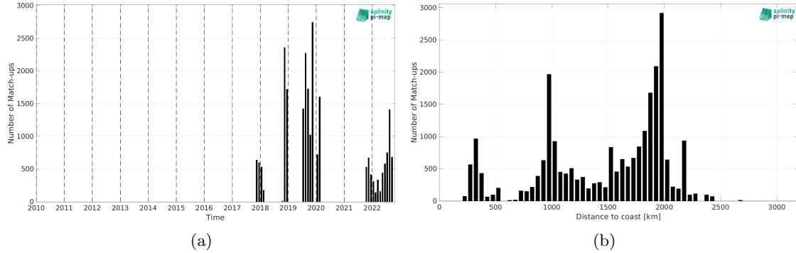
Figure 1: Number of match-ups between Saildrone and SMOS SSS L2Q v331 - 0.25 Deg (CATDS-CPDC) SSS as a function of time (a) and as function of the distance to coast (b) over the Equatorial Ocean 10N-10S Pi-MEP region and for the full satellite product period.
