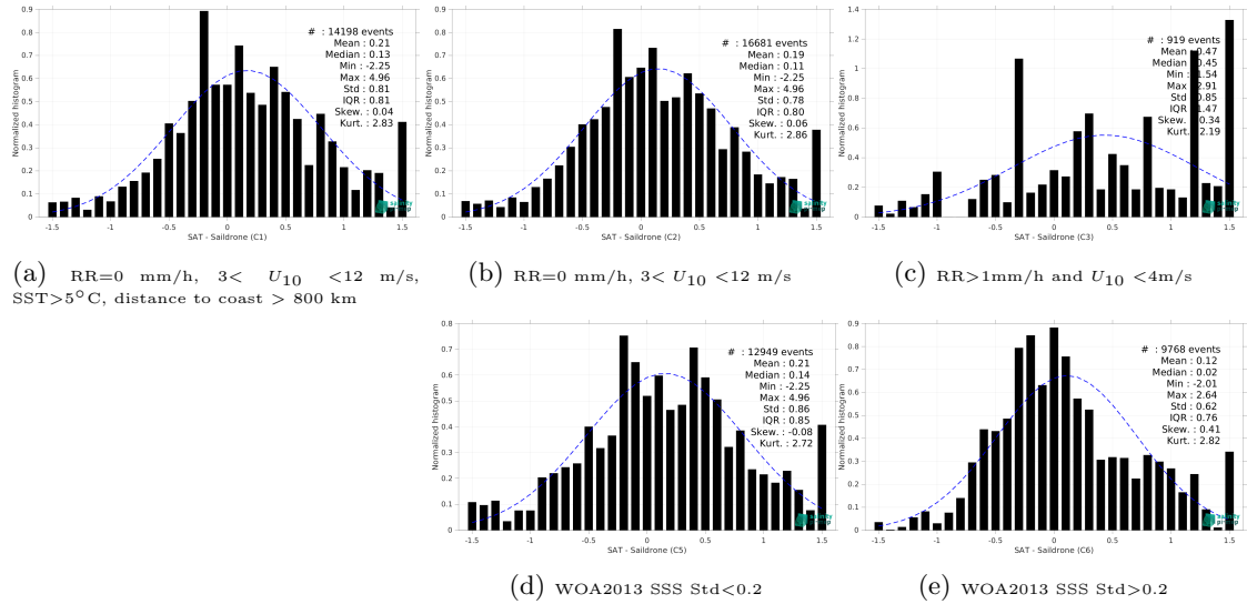
Figure 13: Normalized histogram of \Delta SSS (SMOS SSS L2Q v331 - 0.25 Deg (CATDS-CPDC) - Saildrone) for 5 different subdatasets corresponding to: RR=0 mm/h, 3 < U_{10} < 12 m/s, SST >5^\circ\text{C} , distance to coast > 800 km (a), RR=0 mm/h, 3 < U_{10} < 12 m/s (b), RR >1 mm/h and U_{10} < 4 m/s (c), WOA2013 SSS Std <0.2 (d), WOA2013 SSS Std >0.2 (e).
