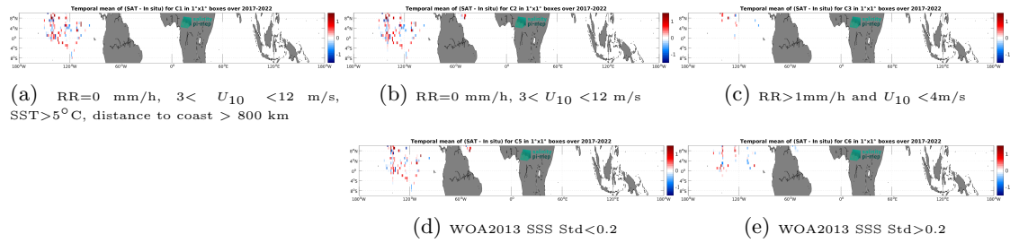
Figure 12: Temporal mean gridded over spatial boxes of size 1^\circ \times 1^\circ of \Delta SSS (SMOS SSS L2Q v331 - 0.25 Deg (CATDS-CPDC) - Saildrone) for 5 different subdatasets corresponding to: RR=0 mm/h, 3 < U_{10} < 12 m/s, SST >5^\circ\text{C} , distance to coast > 800 km (a), RR=0 mm/h, 3 < U_{10} < 12 m/s (b), RR >1 mm/h and U_{10} < 4 m/s (c), WOA2013 SSS Std <0.2 (d), WOA2013 SSS Std >0.2 (e).
