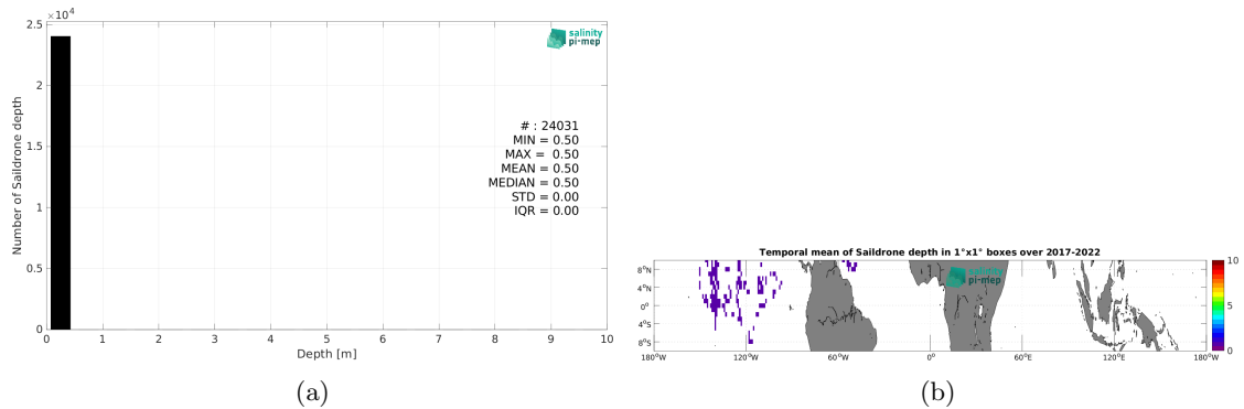
Figure 3: Histograms of the depth of the upper level SSS measurements from Sairdrone in the Match-up DataBase for the Equatorial Ocean 10N-10S Pi-MEP region (a) and temporal mean spatial distribution of pressure of the in situ SSS data over 1^\circ \times 1^\circ boxes and for the full satellite product period (b).
