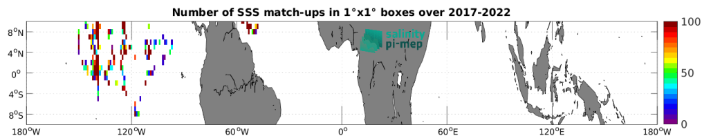
Figure 4: Number of SSS match-ups between Sairdrone SSS and the SMOS SSS L2Q v331 - 0.25 Deg (CATDS-CPDC) SSS product for the Equatorial Ocean 10N-10S Pi-MEP region over 1^\circ \times 1^\circ boxes and for the full satellite product period.
