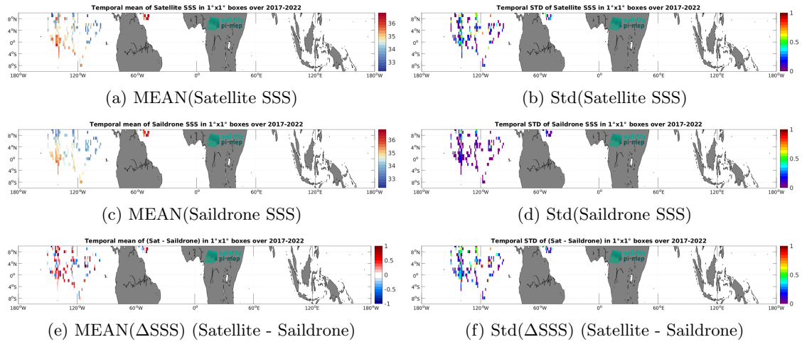
Figure 6: Temporal mean (left) and Std (right) of SSS from SMOS SSS L2Q v331 - 0.25 Deg (CATDS-CPDC) (top), Saildrone (middle), and of \Delta SSS (Satellite - Saildrone). Only match-up pairs are used to generate these maps.
