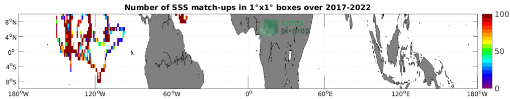
Figure 4: Number of SSS match-ups between Saildrone SSS and the SMOS SSS L2Q v331 - 0.25 Deg (CATDS-CPDC) SSS product for the Equatorial Ocean 10N-10S Pi-MEP region over 1^\circ \times 1^\circ boxes and for the full satellite product period.
