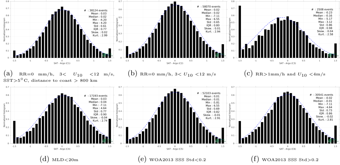
Figure 13: Normalized histogram of \Delta SSS (SMOS SSS L2Q v331 - 0.25 Deg (CATDS-CPDC) - Argo) for 6 different subdatasets corresponding to: RR=0 mm/h, 3 < U_{10} < 12 m/s, SST > 5°C, distance to coast > 800 km (a), RR=0 mm/h, 3 < U_{10} < 12 m/s (b), RR > 1mm/h and U_{10} < 4m/s (c), MLD < 20m (d), WOA2013 SSS Std < 0.2 (e), WOA2013 SSS Std > 0.2 (f).
