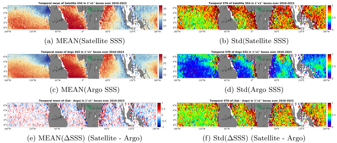
Figure 6: Temporal mean (left) and Std (right) of SSS from SMOS SSS L2Q v331 - 0.25 Deg (CATDS-CPDC) (top), Argo (middle), and of \Delta SSS (Satellite - Argo). Only match-up pairs are used to generate these maps.
