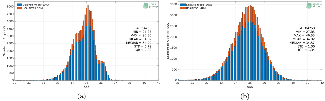
Figure 2: Histograms of SSS from Argo (a) and SMOS SSS L2Q v331 - 0.25 Deg (CATDS-CPDC) (b) considering all match-up pairs per bins of 0.1 over the Equatorial Ocean 10N-10S Pi-MEP region and for the full satellite product period.
