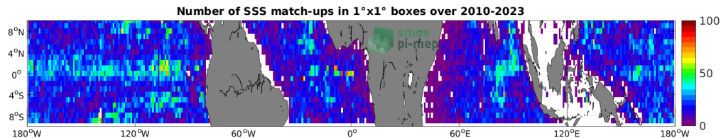
Figure 4: Number of SSS match-ups between Argo SSS and the SMOS SSS L2Q v331 - 0.25 Deg (CATDS-CPDC) SSS product for the Equatorial Ocean 10N-10S Pi-MEP region over 1^\circ \times 1^\circ boxes and for the full satellite product period.
