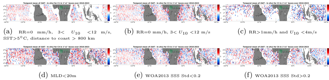
Figure 12: Temporal mean gridded over spatial boxes of size 1^\circ \times 1^\circ of \Delta SSS (SMOS SSS L2Q v331 - 0.25 Deg (CATDS-CPDC) - Argo) for 6 different subdatasets corresponding to:RR=0 mm/h, 3 < U_{10} < 12 m/s, SST >5^\circ C, distance to coast > 800 km (a), RR=0 mm/h, 3 < U_{10} < 12 m/s (b), RR >1 mm/h and U_{10} < 4 m/s (c),MLD <20 m (d),WOA2013 SSS Std <0.2 (e),WOA2013 SSS Std >0.2 (f).
