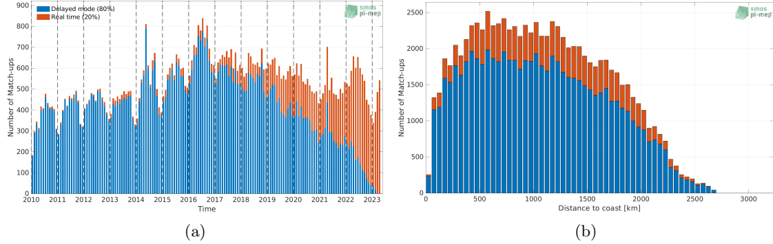
Figure 1: Number of match-ups between Argo and SMOS SSS L2Q v331 - 0.25 Deg (CATDS-CPDC) SSS as a function of time (a) and as function of the distance to coast (b) over the Equatorial Ocean 10N-10S Pi-MEP region and for the full satellite product period.
