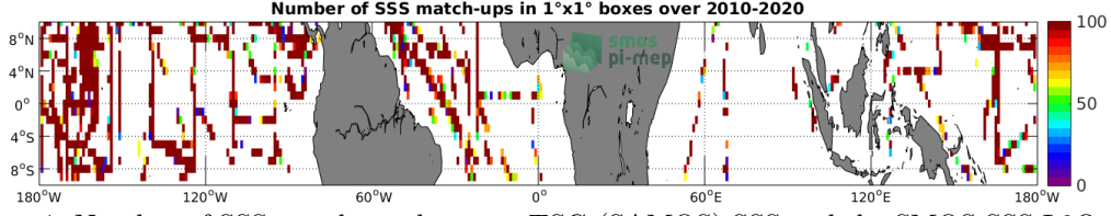
Figure 4: Number of SSS match-ups between TSG (SAMOS) SSS and the SMOS SSS L2Q v330 - 0.25 Deg (CATDS-CPDC) SSS product for the Equatorial Ocean 10N-10S Pi-MEP region over 1^\circ \times 1^\circ boxes and for the full satellite product period.
