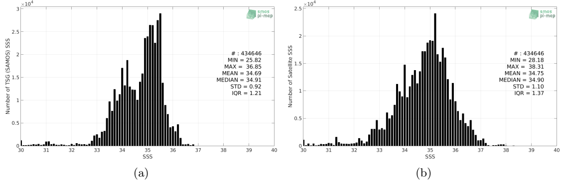
Figure 2: Histograms of SSS from TSG (SAMOS) (a) and SMOS SSS L2Q v330 - 0.25 Deg (CATDS-CPDC) (b) considering all match-up pairs per bins of 0.1 over the Equatorial Ocean 10N-10S Pi-MEP region and for the full satellite product period.
