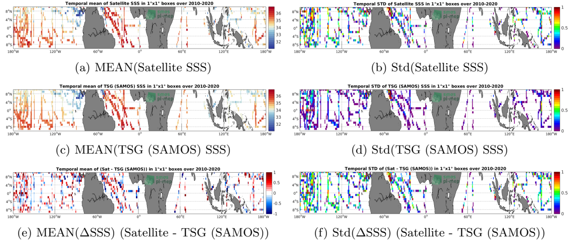
Figure 6: Temporal mean (left) and Std (right) of SSS from SMOS SSS L2Q v330 - 0.25 Deg (CATDS-CPDC) (top), TSG (SAMOS) (middle), and of \Delta SSS (Satellite - TSG (SAMOS)). Only match-up pairs are used to generate these maps.
