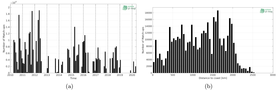
Figure 1: Number of match-ups between TSG (SAMOS) and SMOS SSS L2Q v330 - 0.25 Deg (CATDS-CPDC) SSS as a function of time (a) and as function of the distance to coast (b) over the Equatorial Ocean 10N-10S Pi-MEP region and for the full satellite product period.
