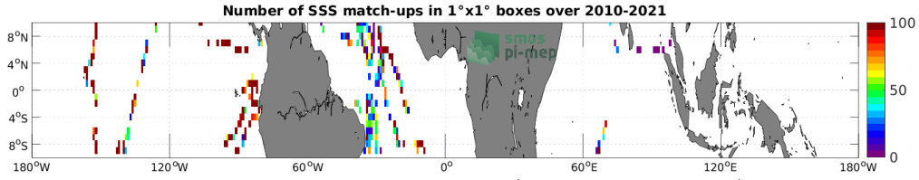
Figure 4: Number of SSS match-ups between TSG (GOSUD-Sailing-ship) SSS and the SMOS SSS L2Q v330 - 0.25 Deg (CATDS-CPDC) SSS product for the Equatorial Ocean 10N-10S Pi-MEP region over 1^\circ \times 1^\circ boxes and for the full satellite product period.
