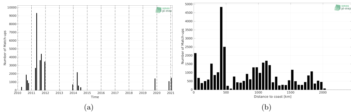
Figure 1: Number of match-ups between TSG (GOSUD-Sailing-ship) and SMOS SSS L2Q v330 - 0.25 Deg (CATDS-CPDC) SSS as a function of time (a) and as function of the distance to coast (b) over the Equatorial Ocean 10N-10S Pi-MEP region and for the full satellite product period.
