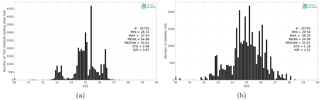
Figure 2: Histograms of SSS from TSG (GOSUD-Sailing-ship) (a) and SMOS SSS L2Q v330 - 0.25 Deg (CATDS-CPDC) (b) considering all match-up pairs per bins of 0.1 over the Equatorial Ocean 10N-10S Pi-MEP region and for the full satellite product period.
