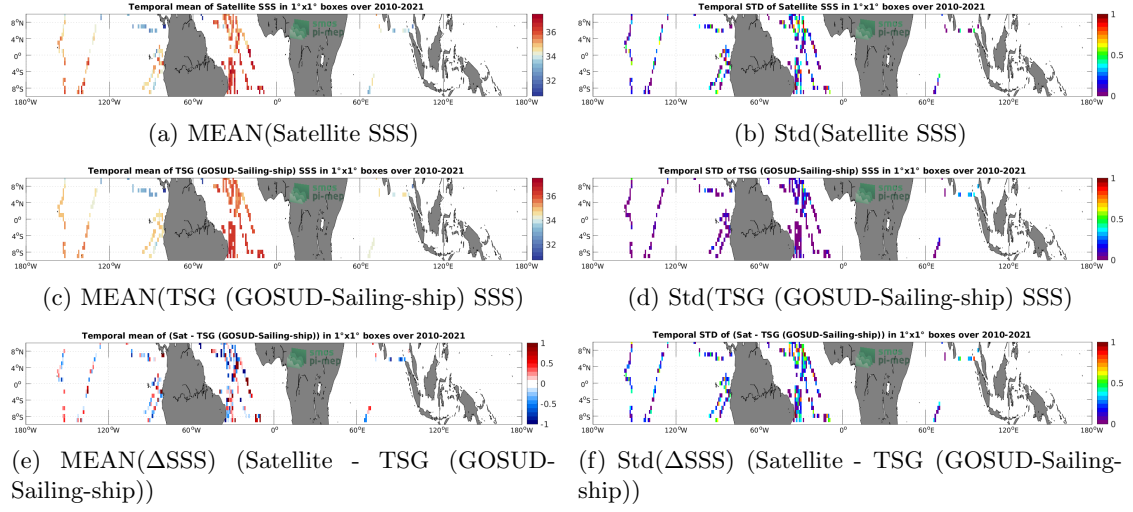
Figure 6: Temporal mean (left) and Std (right) of SSS from SMOS SSS L2Q v330 - 0.25 Deg (CATDS-CPDC) (top), TSG (GOSUD-Sailing-ship) (middle), and of \Delta SSS (Satellite - TSG (GOSUD-Sailing-ship)). Only match-up pairs are used to generate these maps.
