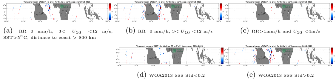
Figure 12: Temporal mean gridded over spatial boxes of size 1^{\circ}\times 1^{\circ} of \Delta SSS (SMOS SSS L2Q v330 - 0.25 Deg (CATDS-CPDC) - TSG (GOSUD-Sailing-ship)) for 5 different subdatasets corresponding to:RR=0 mm/h, 3 < U_{10} < 12 m/s, SST > 5^{\circ}\text{C} , distance to coast > 800 km (a), RR=0 mm/h, 3 < U_{10} < 12 m/s (b), RR > 1 mm/h and U_{10} < 4 m/s (c), WOA2013 SSS Std < 0.2 (d), WOA2013 SSS Std > 0.2 (e).
