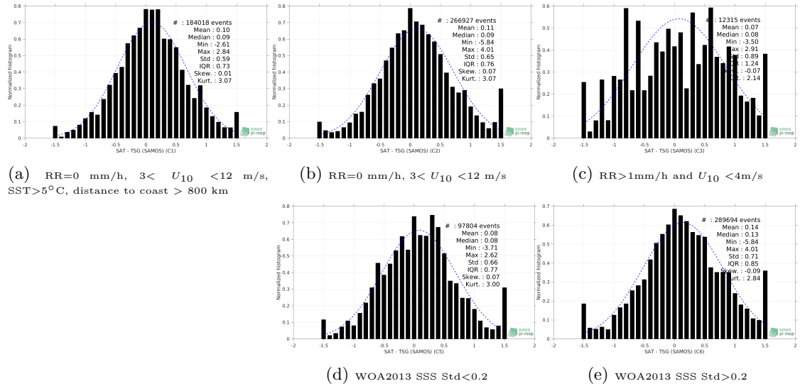
Figure 13: Normalized histogram of \Delta SSS (SMOS SSS L2Q v321 - 0.25 Deg (CATDS-CPDC) - TSG (SAMOS)) for 5 different subdatasets corresponding to: RR=0 mm/h, 3 < U_{10} < 12 m/s, SST >5^\circ\text{C} , distance to coast > 800 km (a), RR=0 mm/h, 3 < U_{10} < 12 m/s (b), RR >1 mm/h and U_{10} < 4 m/s (c), WOA2013 SSS Std <0.2 (d), WOA2013 SSS Std >0.2 (e).
