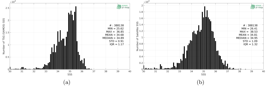
Figure 2: Histograms of SSS from TSG (SAMOS) (a) and SMOS SSS L2Q v321 - 0.25 Deg (CATDS-CPDC) (b) considering all match-up pairs per bins of 0.1 over the Equatorial Ocean 10N-10S Pi-MEP region and for the full satellite product period.
