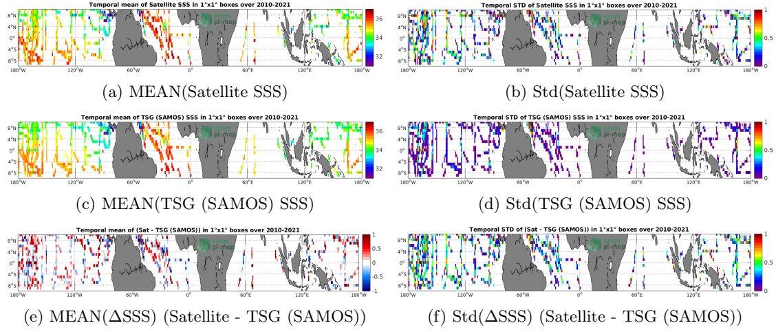
Figure 6: Temporal mean (left) and Std (right) of SSS from SMOS SSS L2Q v321 - 0.25 Deg (CATDS-CPDC) (top), TSG (SAMOS) (middle), and of \Delta SSS (Satellite - TSG (SAMOS)). Only match-up pairs are used to generate these maps.
