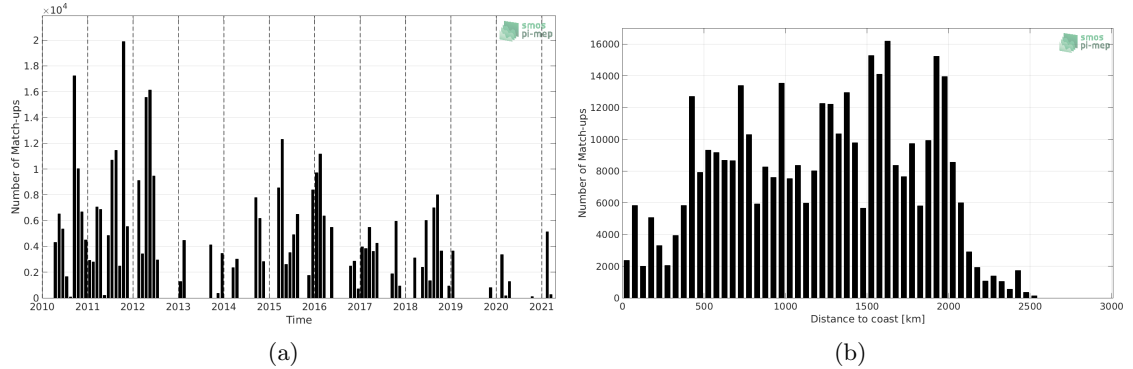
Figure 1: Number of match-ups between TSG (SAMOS) and SMOS SSS L2Q v321 - 0.25 Deg (CATDS-CPDC) SSS as a function of time (a) and as function of the distance to coast (b) over the Equatorial Ocean 10N-10S Pi-MEP region and for the full satellite product period.
