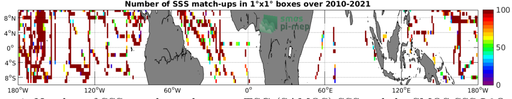
Figure 4: Number of SSS match-ups between TSG (SAMOS) SSS and the SMOS SSS L2Q v321 - 0.25 Deg (CATDS-CPDC) SSS product for the Equatorial Ocean 10N-10S Pi-MEP region over 1^\circ \times 1^\circ boxes and for the full satellite product period.
