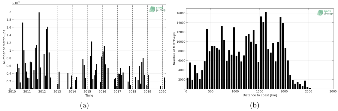
Figure 1: Number of match-ups between TSG-SAMOS and SMOS L2Q v321 - 0.25 Deg (CATDS-CPDC) SSS as a function of time (a) and as function of the distance to coast (b) over the Equatorial Ocean 10N-10S Pi-MEP region and for the full satellite product period.
