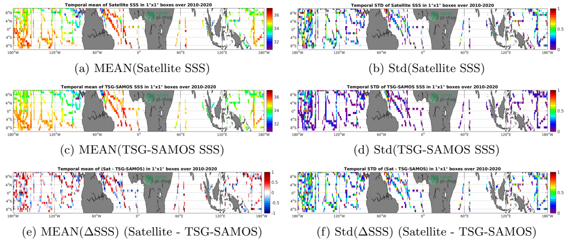
Figure 6: Temporal mean (left) and Std (right) of SSS from SMOS L2Q v321 - 0.25 Deg (CATDS-CPDC) (top), TSG-SAMOS (middle), and of \Delta SSS (Satellite - TSG-SAMOS). Only match-up pairs are used to generate these maps.
