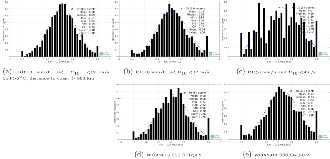
Figure 13: Normalized histogram of \Delta SSS (SMOS L2Q v321 - 0.25 Deg (CATDS-CPDC) - TSG-SAMOS) for 5 different subdatasets corresponding to: RR=0 mm/h, 3 < U_{10} < 12 m/s, SST > 5^\circ C , distance to coast > 800 km (a), RR=0 mm/h, 3 < U_{10} < 12 m/s (b), RR > 1 mm/h and U_{10} < 4 m/s (c), WOA2013 SSS Std < 0.2 (d), WOA2013 SSS Std > 0.2 (e).
