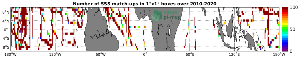
Figure 4: Number of SSS match-ups between TSG-SAMOS SSS and the SMOS L2Q v321 - 0.25 Deg (CATDS-CPDC) SSS product for the Equatorial Ocean 10N-10S Pi-MEP region over 1^\circ \times 1^\circ boxes and for the full satellite product period.
