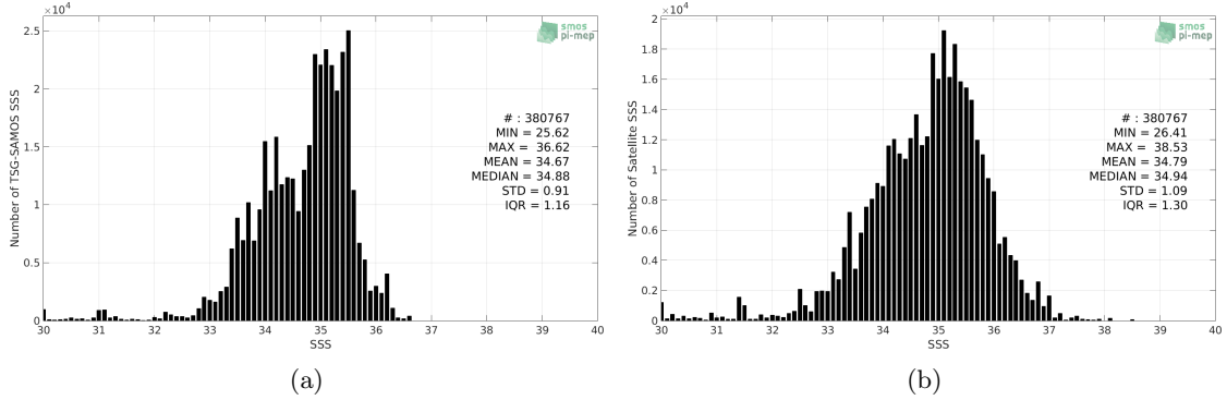
Figure 2: Histograms of SSS from TSG-SAMOS (a) and SMOS L2Q v321 - 0.25 Deg (CATDS-CPDC) (b) considering all match-up pairs per bins of 0.1 over the Equatorial Ocean 10N-10S Pi-MEP region and for the full satellite product period.
