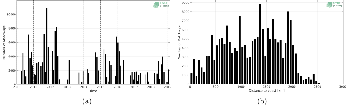
Figure 1: Number of match-ups between TSG-SAMOS and SMOS-L3-CATDS-CPDC-V321-L2Q SSS as a function of time (a) and as function of the distance to coast (b) over the Equatorial Ocean 10N-10S Pi-MEP region and for the full satellite product period.
