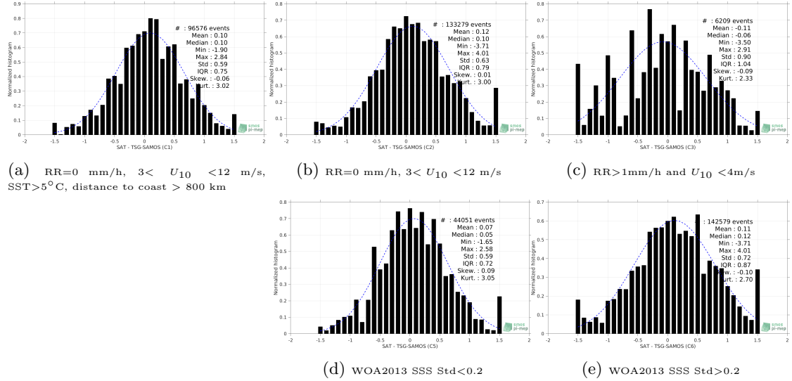
Figure 13: Normalized histogram of \Delta SSS (SMOS-L3-CATDS-CPDC-V321-L2Q - TSG-SAMOS) for 5 different subdatasets corresponding to: RR=0 mm/h, 3 < U_{10} < 12 m/s, SST >5^\circ C, distance to coast > 800 km (a), RR=0 mm/h, 3 < U_{10} < 12 m/s (b), RR >1 mm/h and U_{10} < 4 m/s (c), WOA2013 SSS Std <0.2 (d), WOA2013 SSS Std >0.2 (e).
