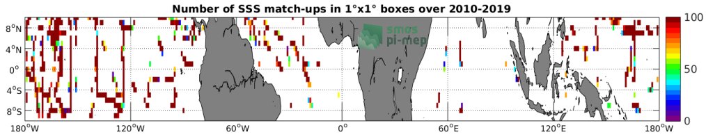
Figure 4: Number of SSS match-ups between TSG-SAMOS SSS and the SMOS-L3-CATDS-CPDC-V321-L2Q SSS product for the Equatorial Ocean 10N-10S Pi-MEP region over 1^\circ \times 1^\circ boxes and for the full satellite product period.
