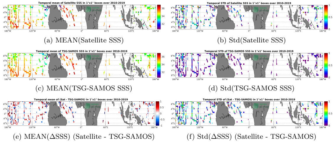
Figure 6: Temporal mean (left) and Std (right) of SSS from SMOS-L3-CATDS-CPDC-V321-L2Q (top), TSG-SAMOS (middle), and of \Delta SSS (Satellite - TSG-SAMOS). Only match-up pairs are used to generate these maps.
