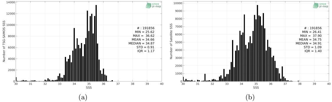
Figure 2: Histograms of SSS from TSG-SAMOS (a) and SMOS-L3-CATDS-CPDC-V321-L2Q (b) considering all match-up pairs per bins of 0.1 over the Equatorial Ocean 10N-10S Pi-MEP region and for the full satellite product period.
