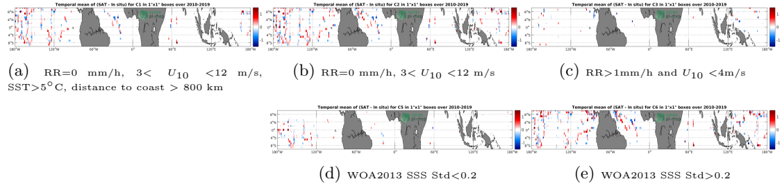
Figure 12: Temporal mean gridded over spatial boxes of size 1^\circ \times 1^\circ of \Delta SSS (SMOS-L3-CATDS-CPDC-V321-L2Q - TSG-SAMOS) for 5 different subdatasets corresponding to:RR=0 mm/h, 3 < U_{10} < 12 m/s, SST >5^\circ C, distance to coast > 800 km (a), RR=0 mm/h, 3 < U_{10} < 12 m/s (b), RR >1 mm/h and U_{10} < 4 m/s (c), WOA2013 SSS Std <0.2 (d), WOA2013 SSS Std >0.2 (e).
