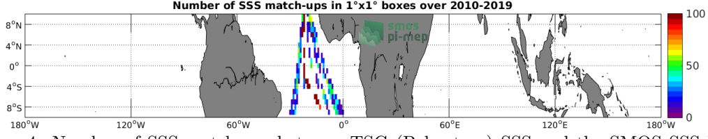
Figure 4: Number of SSS match-ups between TSG (Polarstern) SSS and the SMOS SSS L2Q v321 - 0.25 Deg (CATDS-CPDC) SSS product for the Equatorial Ocean 10N-10S Pi-MEP region over 1^\circ \times 1^\circ boxes and for the full satellite product period.
