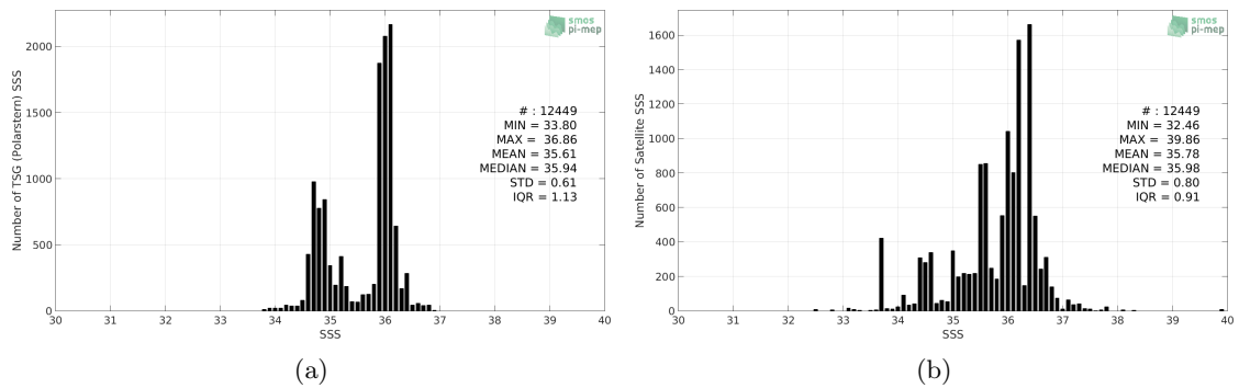
Figure 2: Histograms of SSS from TSG (Polarstern) (a) and SMOS SSS L2Q v321 - 0.25 Deg (CATDS-CPDC) (b) considering all match-up pairs per bins of 0.1 over the Equatorial Ocean 10N-10S Pi-MEP region and for the full satellite product period.
