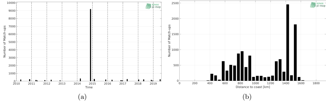
Figure 1: Number of match-ups between TSG (Polarstern) and SMOS SSS L2Q v321 - 0.25 Deg (CATDS-CPDC) SSS as a function of time (a) and as function of the distance to coast (b) over the Equatorial Ocean 10N-10S Pi-MEP region and for the full satellite product period.
