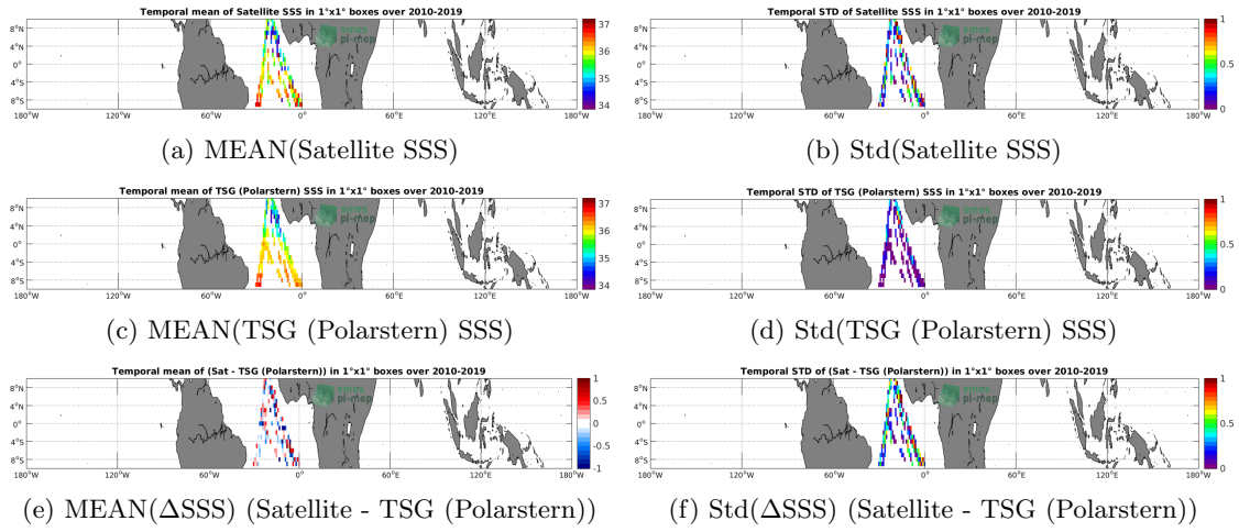
Figure 6: Temporal mean (left) and Std (right) of SSS from SMOS SSS L2Q v321 - 0.25 Deg (CATDS-CPDC) (top), TSG (Polarstern) (middle), and of \Delta SSS (Satellite - TSG (Polarstern)). Only match-up pairs are used to generate these maps.
