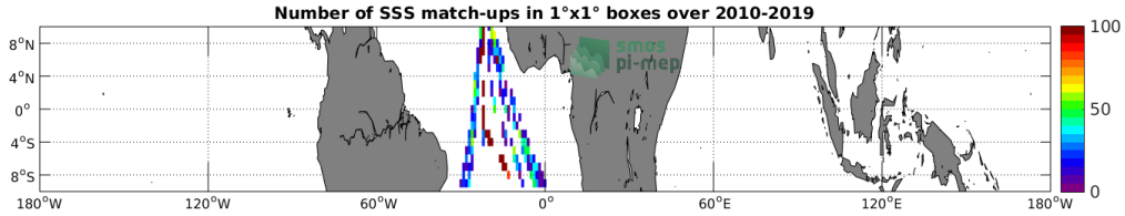
Figure 4: Number of SSS match-ups between TSG (Polarstern) SSS and the SMOS SSS L2Q v321 - 0.25 Deg (CATDS-CPDC) SSS product for the Equatorial Ocean 10N-10S Pi-MEP region over 1°x1° boxes and for the full satellite product period.
