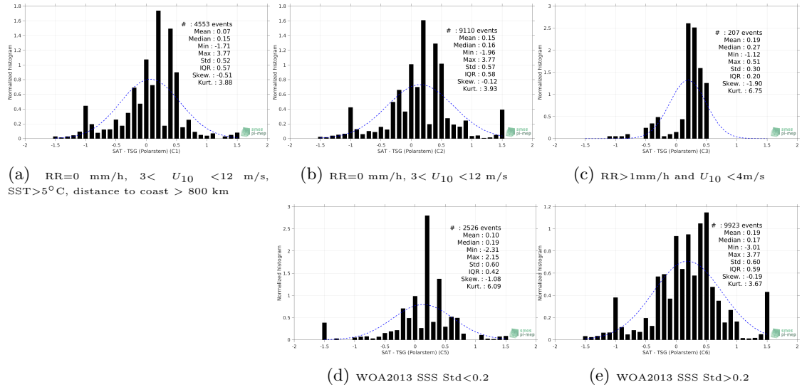
Figure 13: Normalized histogram of \Delta SSS (SMOS SSS L2Q v321 - 0.25 Deg (CATDS-CPDC) - TSG (Polarstern)) for 5 different subdatasets corresponding to: RR=0 mm/h, 3 < U_{10} < 12 m/s, SST >5^\circ\text{C} , distance to coast > 800 km (a), RR=0 mm/h, 3 < U_{10} < 12 m/s (b), RR >1 mm/h and U_{10} < 4 m/s (c), WOA2013 SSS Std <0.2 (d), WOA2013 SSS Std >0.2 (e).
