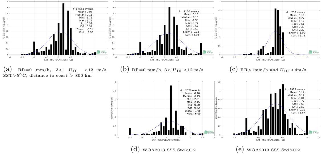
Figure 13: Normalized histogram of \Delta SSS (SMOS L2Q v321 - 0.25 Deg (CATDS-CPDC) - TSG-POLARSTERN) for 5 different subdatasets corresponding to: RR=0 mm/h, 3 < U_{10} < 12 m/s, SST > 5^\circ C , distance to coast > 800 km (a), RR=0 mm/h, 3 < U_{10} < 12 m/s (b), RR > 1 mm/h and U_{10} < 4 m/s (c), WOA2013 SSS Std < 0.2 (d), WOA2013 SSS Std > 0.2 (e).
