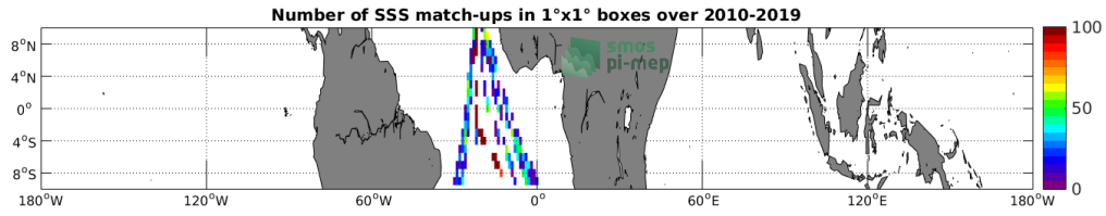
Figure 4: Number of SSS match-ups between TSG-POLARSTERN SSS and the SMOS L2Q v321 - 0.25 Deg (CATDS-CPDC) SSS product for the Equatorial Ocean 10N-10S Pi-MEP region over 1^\circ \times 1^\circ boxes and for the full satellite product period.
