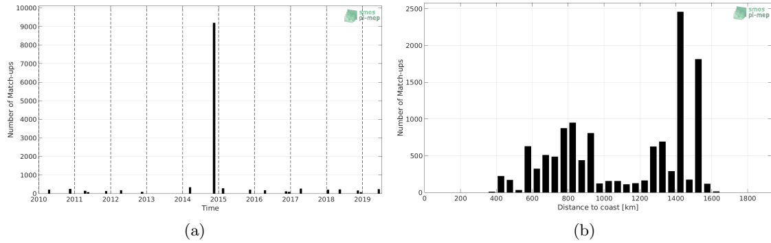
Figure 1: Number of match-ups between TSG-POLARSTERN and SMOS L2Q v321 - 0.25 Deg (CATDS-CPDC) SSS as a function of time (a) and as function of the distance to coast (b) over the Equatorial Ocean 10N-10S Pi-MEP region and for the full satellite product period.
