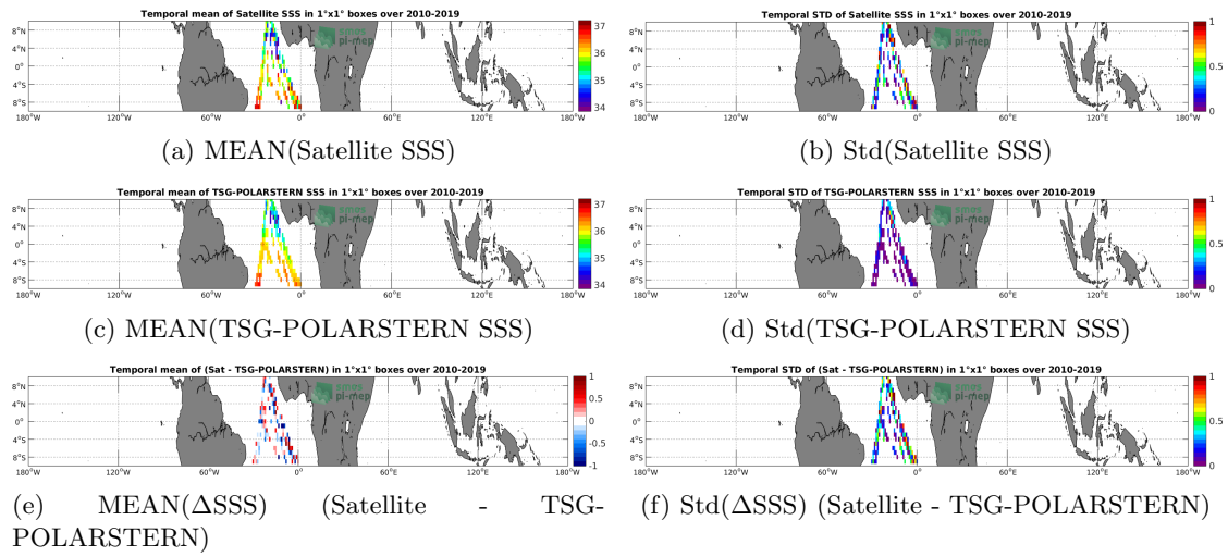
Figure 6: Temporal mean (left) and Std (right) of SSS from SMOS L2Q v321 - 0.25 Deg (CATDS-CPDC) (top), TSG-POLARSTERN (middle), and of \Delta SSS (Satellite - TSG-POLARSTERN). Only match-up pairs are used to generate these maps.
