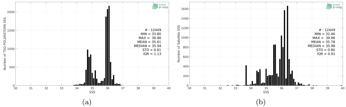
Figure 2: Histograms of SSS from TSG-POLARSTERN (a) and SMOS L2Q v321 - 0.25 Deg (CATDS-CPDC) (b) considering all match-up pairs per bins of 0.1 over the Equatorial Ocean 10N-10S Pi-MEP region and for the full satellite product period.
