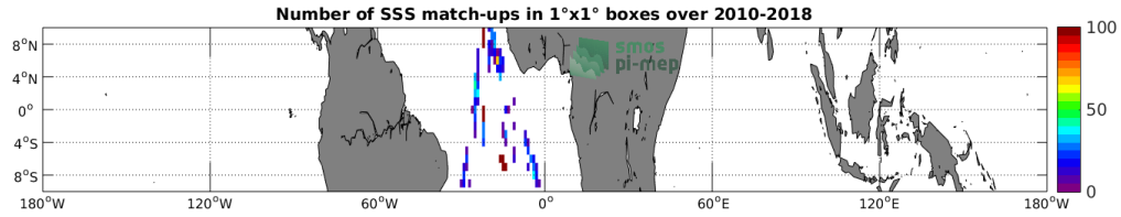
Figure 4: Number of SSS match-ups between TSG-POLARSTERN SSS and the SMOS-L3-CATDS-CPDC-V321-L2Q SSS product for the Equatorial Ocean 10N-10S Pi-MEP region over 1^\circ \times 1^\circ boxes and for the full satellite product period.
