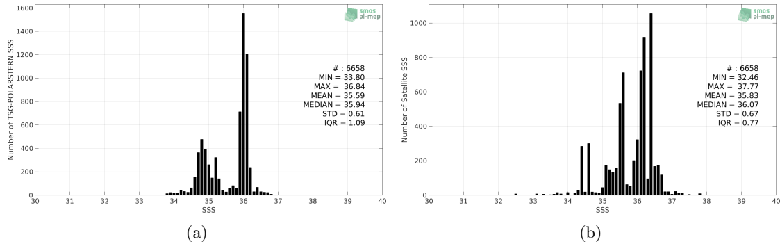
Figure 2: Histograms of SSS from TSG-POLARSTERN (a) and SMOS-L3-CATDS-CPDC-V321-L2Q (b) considering all match-up pairs per bins of 0.1 over the Equatorial Ocean 10N-10S Pi-MEP region and for the full satellite product period.
