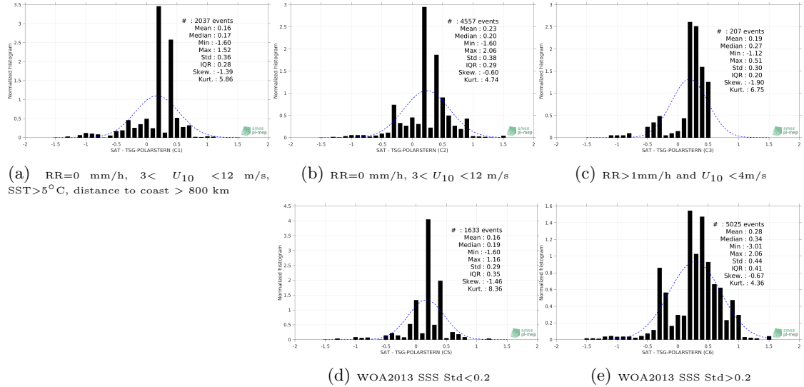
Figure 13: Normalized histogram of \Delta SSS (SMOS-L3-CATDS-CPDC-V321-L2Q - TSG-POLARSTERN) for 5 different subdatasets corresponding to: RR=0 mm/h, 3 < U_{10} < 12 m/s, SST >5^\circ\text{C} , distance to coast > 800 km (a), RR=0 mm/h, 3 < U_{10} < 12 m/s (b), RR >1 mm/h and U_{10} < 4 m/s (c), WOA2013 SSS Std <0.2 (d), WOA2013 SSS Std >0.2 (e).
