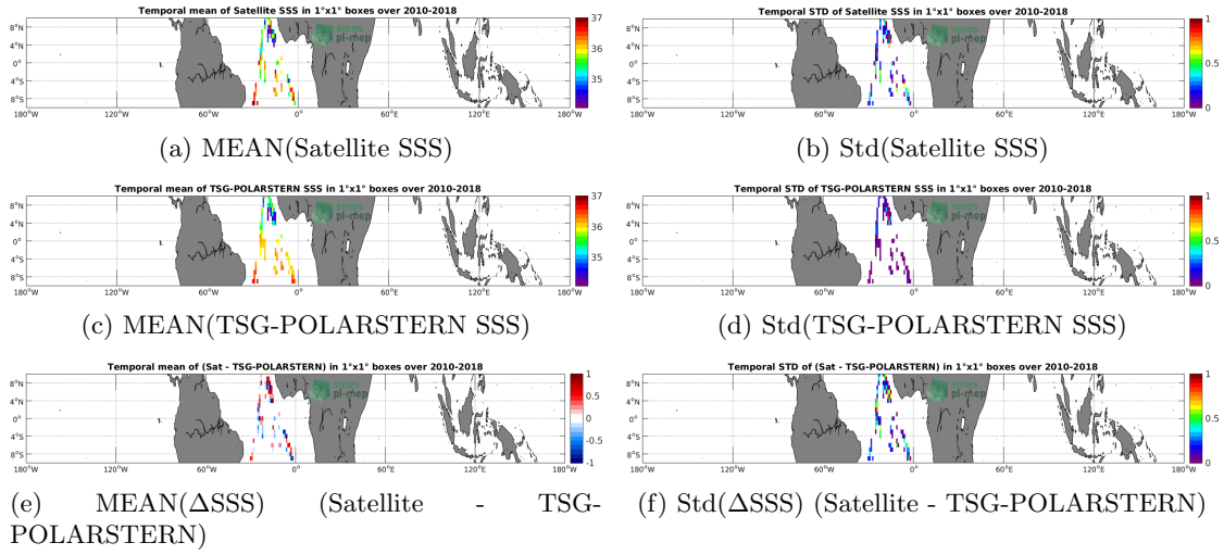
Figure 6: Temporal mean (left) and Std (right) of SSS from SMOS-L3-CATDS-CPDC-V321-L2Q (top), TSG-POLARSTERN (middle), and of \Delta SSS (Satellite - TSG-POLARSTERN). Only match-up pairs are used to generate these maps.
