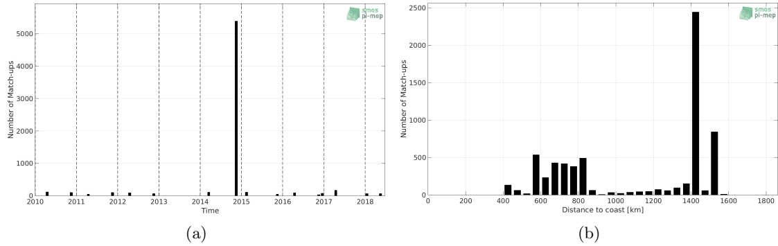
Figure 1: Number of match-ups between TSG-POLARSTERN and SMOS-L3-CATDS-CPDC-V321-L2Q SSS as a function of time (a) and as function of the distance to coast (b) over the Equatorial Ocean 10N-10S Pi-MEP region and for the full satellite product period.
