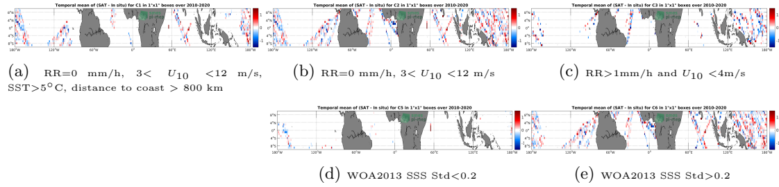
Figure 12: Temporal mean gridded over spatial boxes of size 1^{\circ}\times 1^{\circ} of \Delta\text{SSS} (SMOS SSS L2Q v321 - 0.25 Deg (CATDS-CPDC) - TSG (LEGOS-DM)) for 5 different subdatasets corresponding to: \text{RR}=0 mm/h, 3 < U_{10} < 12 m/s, SST > 5^{\circ}\text{C} , distance to coast > 800 km (a), \text{RR}=0 mm/h, 3 < U_{10} < 12 m/s (b), \text{RR} > 1 mm/h and U_{10} < 4 m/s (c), WOA2013 SSS Std < 0.2 (d), WOA2013 SSS Std > 0.2 (e).
