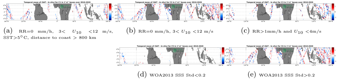
Figure 12: Temporal mean gridded over spatial boxes of size 1^{\circ}\times 1^{\circ} of \Delta\text{SSS} (SMOS SSS L2Q v321 - 0.25 Deg (CATDS-CPDC) - TSG (LEGOS-DM)) for 5 different subdatasets corresponding to:RR=0 mm/h, 3 < U_{10} < 12 m/s, SST >5^{\circ}\text{C} , distance to coast > 800 km (a), RR=0 mm/h, 3 < U_{10} < 12 m/s (b), RR >1 mm/h and U_{10} < 4 m/s (c), WOA2013 SSS Std <0.2 (d), WOA2013 SSS Std >0.2 (e).
