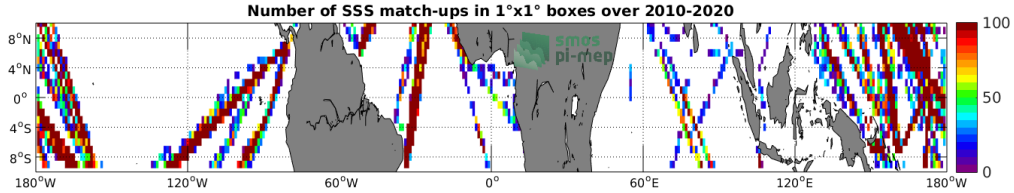
Figure 4: Number of SSS match-ups between TSG (LEGOS-DM) SSS and the SMOS SSS L2Q v321 - 0.25 Deg (CATDS-CPDC) SSS product for the Equatorial Ocean 10N-10S Pi-MEP region over 1^\circ \times 1^\circ boxes and for the full satellite product period.
