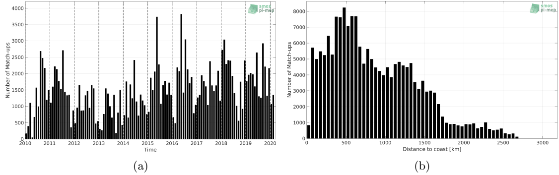
Figure 1: Number of match-ups between TSG (LEGOS-DM) and SMOS SSS L2Q v321 - 0.25 Deg (CATDS-CPDC) SSS as a function of time (a) and as function of the distance to coast (b) over the Equatorial Ocean 10N-10S Pi-MEP region and for the full satellite product period.
