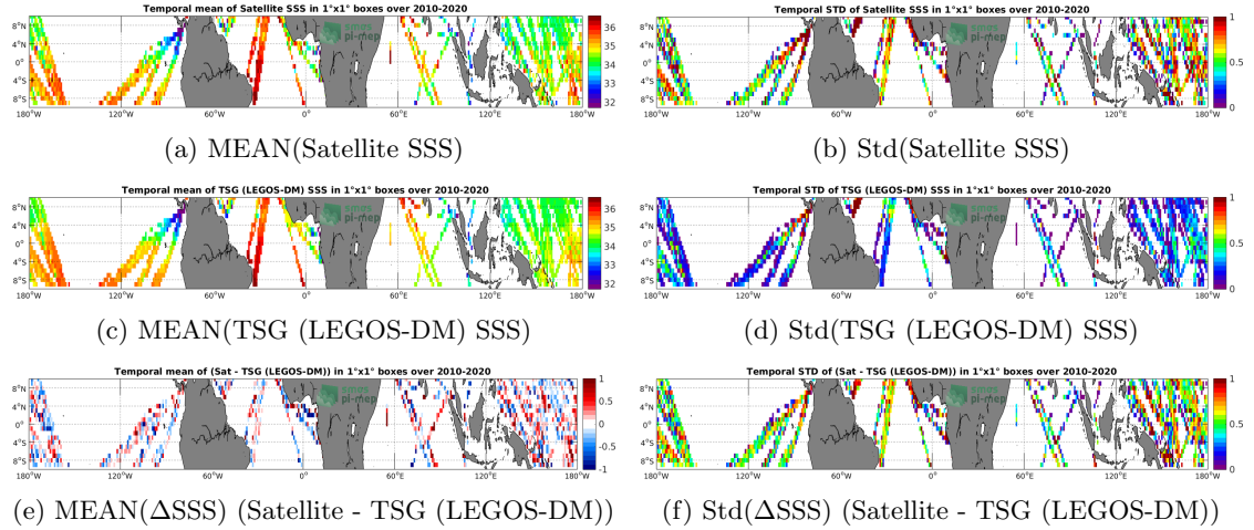
Figure 6: Temporal mean (left) and Std (right) of SSS from SMOS SSS L2Q v321 - 0.25 Deg (CATDS-CPDC) (top), TSG (LEGOS-DM) (middle), and of \Delta SSS (Satellite - TSG (LEGOS-DM)). Only match-up pairs are used to generate these maps.
