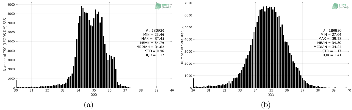
Figure 2: Histograms of SSS from TSG (LEGOS-DM) (a) and SMOS SSS L2Q v321 - 0.25 Deg (CATDS-CPDC) (b) considering all match-up pairs per bins of 0.1 over the Equatorial Ocean 10N-10S Pi-MEP region and for the full satellite product period.
