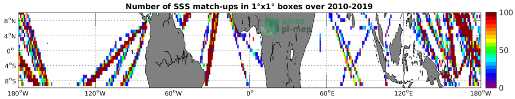
Figure 4: Number of SSS match-ups between TSG (LEGOS-DM) SSS and the SMOS SSS L2Q v321 - 0.25 Deg (CATDS-CPDC) SSS product for the Equatorial Ocean 10N-10S Pi-MEP region over 1°x1° boxes and for the full satellite product period.
