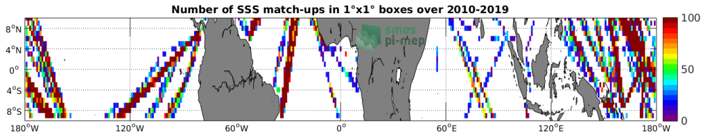
Figure 4: Number of SSS match-ups between TSG-LEGOS-DM SSS and the SMOS L2Q v321 - 0.25 Deg (CATDS-CPDC) SSS product for the Equatorial Ocean 10N-10S Pi-MEP region over 1°x1° boxes and for the full satellite product period.
