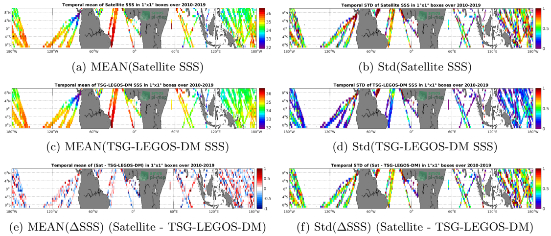
Figure 6: Temporal mean (left) and Std (right) of SSS from SMOS L2Q v321 - 0.25 Deg (CATDS-CPDC) (top), TSG-LEGOS-DM (middle), and of \Delta SSS (Satellite - TSG-LEGOS-DM). Only match-up pairs are used to generate these maps.
