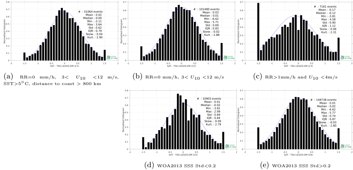
Figure 13: Normalized histogram of \Delta SSS (SMOS L2Q v321 - 0.25 Deg (CATDS-CPDC) - TSG-LEGOS-DM) for 5 different subdatasets corresponding to: RR=0 mm/h, 3 < U_{10} < 12 m/s, SST > 5^\circ C , distance to coast > 800 km (a), RR=0 mm/h, 3 < U_{10} < 12 m/s (b), RR > 1 mm/h and U_{10} < 4 m/s (c), WOA2013 SSS Std < 0.2 (d), WOA2013 SSS Std > 0.2 (e).
