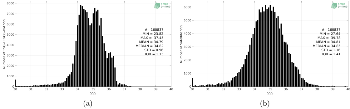
Figure 2: Histograms of SSS from TSG-LEGOS-DM (a) and SMOS L2Q v321 - 0.25 Deg (CATDS-CPDC) (b) considering all match-up pairs per bins of 0.1 over the Equatorial Ocean 10N-10S Pi-MEP region and for the full satellite product period.
