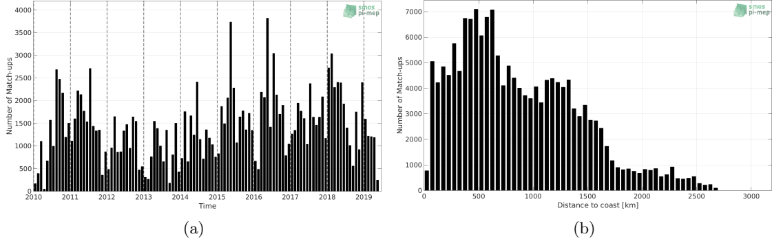
Figure 1: Number of match-ups between TSG-LEGOS-DM and SMOS L2Q v321 - 0.25 Deg (CATDS-CPDC) SSS as a function of time (a) and as function of the distance to coast (b) over the Equatorial Ocean 10N-10S Pi-MEP region and for the full satellite product period.
