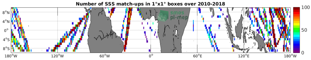
Figure 4: Number of SSS match-ups between TSG-LEGOS-DM SSS and the SMOS-L3-CATDS-CPDC-V321-L2Q SSS product for the Equatorial Ocean 10N-10S Pi-MEP region over 1^\circ \times 1^\circ boxes and for the full satellite product period.
