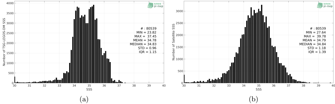
Figure 2: Histograms of SSS from TSG-LEGOS-DM (a) and SMOS-L3-CATDS-CPDC-V321-L2Q (b) considering all match-up pairs per bins of 0.1 over the Equatorial Ocean 10N-10S Pi-MEP region and for the full satellite product period.
