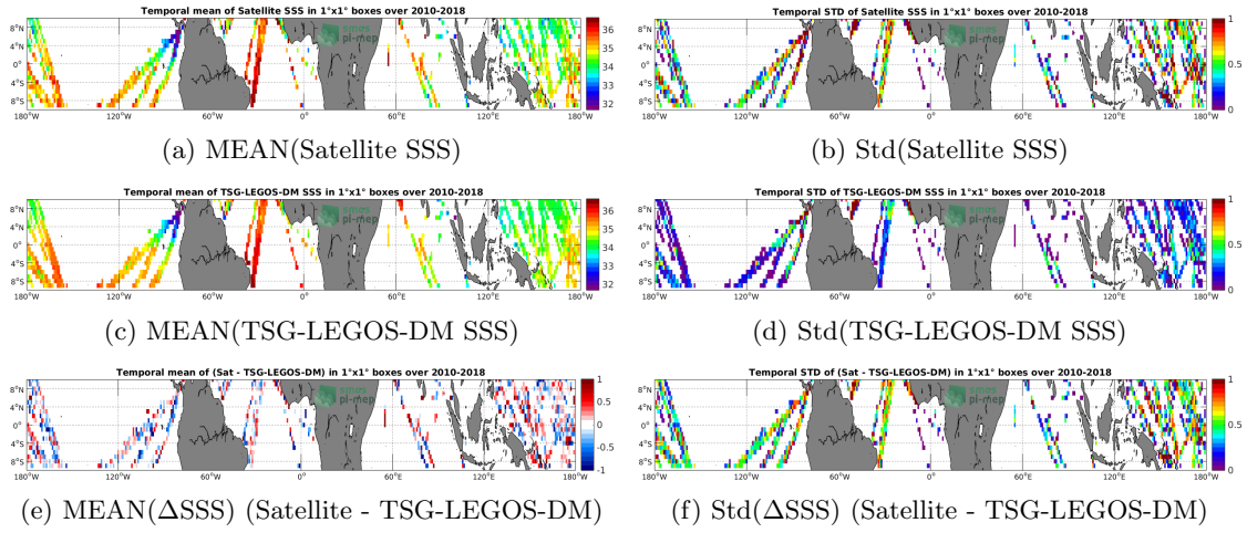
Figure 6: Temporal mean (left) and Std (right) of SSS from SMOS-L3-CATDS-CPDC-V321-L2Q (top), TSG-LEGOS-DM (middle), and of \Delta SSS (Satellite - TSG-LEGOS-DM). Only match-up pairs are used to generate these maps.
