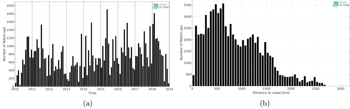
Figure 1: Number of match-ups between TSG-LEGOS-DM and SMOS-L3-CATDS-CPDC-V321-L2Q SSS as a function of time (a) and as function of the distance to coast (b) over the Equatorial Ocean 10N-10S Pi-MEP region and for the full satellite product period.
