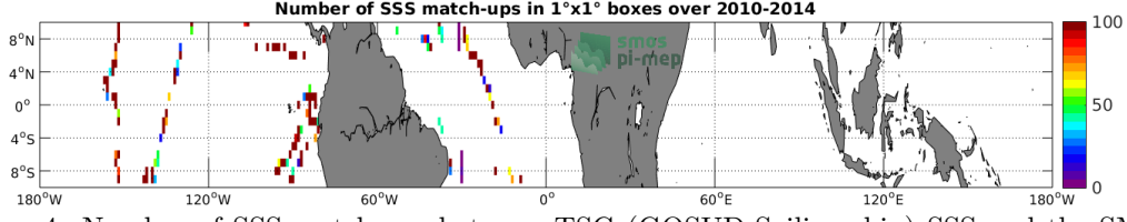
Figure 4: Number of SSS match-ups between TSG (GOSUD-Sailing-ship) SSS and the SMOS SSS L2Q v321 - 0.25 Deg (CATDS-CPDC) SSS product for the Equatorial Ocean 10N-10S Pi-MEP region over 1^\circ \times 1^\circ boxes and for the full satellite product period.
