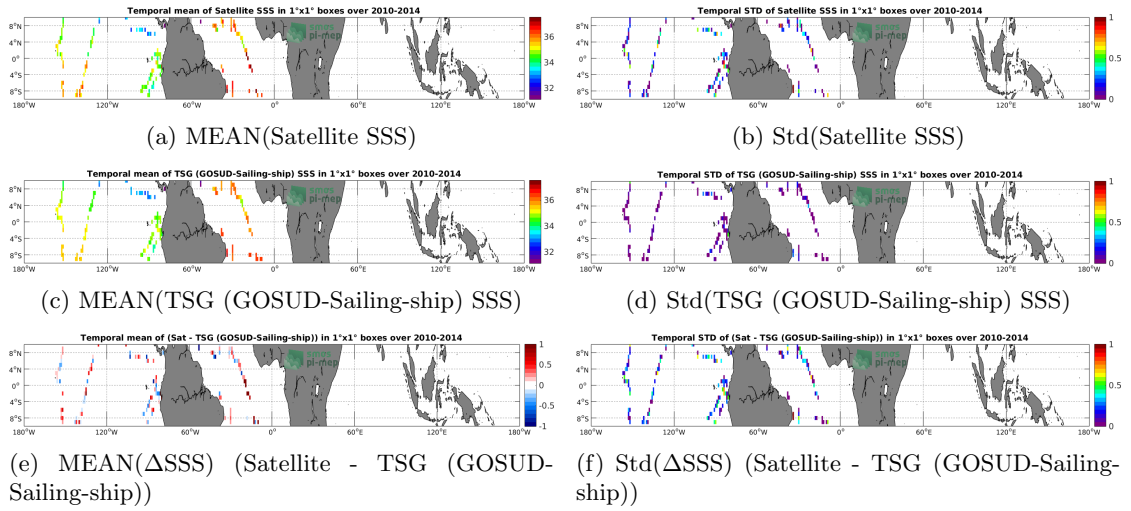
Figure 6: Temporal mean (left) and Std (right) of SSS from SMOS SSS L2Q v321 - 0.25 Deg (CATDS-CPDC) (top), TSG (GOSUD-Sailing-ship) (middle), and of \Delta SSS (Satellite - TSG (GOSUD-Sailing-ship)). Only match-up pairs are used to generate these maps.
