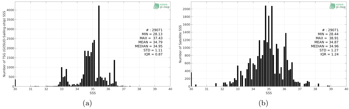
Figure 2: Histograms of SSS from TSG (GOSUD-Sailing-ship) (a) and SMOS SSS L2Q v321 - 0.25 Deg (CATDS-CPDC) (b) considering all match-up pairs per bins of 0.1 over the Equatorial Ocean 10N-10S Pi-MEP region and for the full satellite product period.
