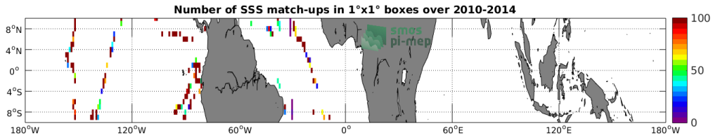
Figure 4: Number of SSS match-ups between TSG (GOSUD-Sailing-ship) SSS and the SMOS SSS L2Q v321 - 0.25 Deg (CATDS-CPDC) SSS product for the Equatorial Ocean 10N-10S Pi-MEP region over 1^\circ \times 1^\circ boxes and for the full satellite product period.
