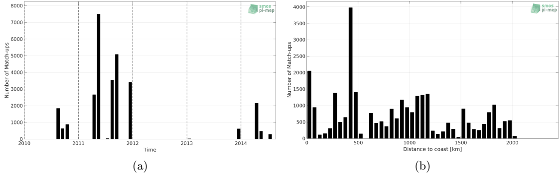
Figure 1: Number of match-ups between TSG (GOSUD-Sailing-ship) and SMOS SSS L2Q v321 - 0.25 Deg (CATDS-CPDC) SSS as a function of time (a) and as function of the distance to coast (b) over the Equatorial Ocean 10N-10S Pi-MEP region and for the full satellite product period.
