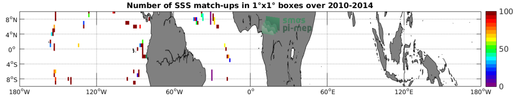
Figure 4: Number of SSS match-ups between TSG-GOSUD-Sailing-ship SSS and the SMOS-L3-CATDS-CPDC-V321-L2Q SSS product for the Equatorial Ocean 10N-10S Pi-MEP region over 1^\circ \times 1^\circ boxes and for the full satellite product period.
