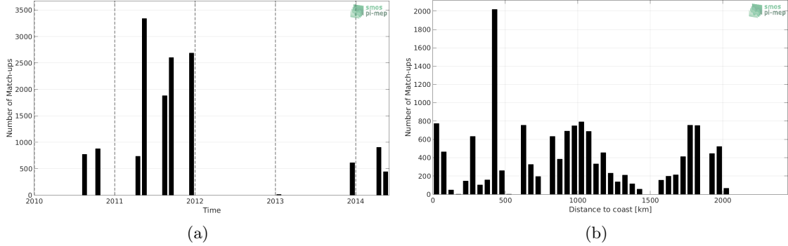
Figure 1: Number of match-ups between TSG-GOSUD-Sailing-ship and SMOS-L3-CATDS-CPDC-V321-L2Q SSS as a function of time (a) and as function of the distance to coast (b) over the Equatorial Ocean 10N-10S Pi-MEP region and for the full satellite product period.
