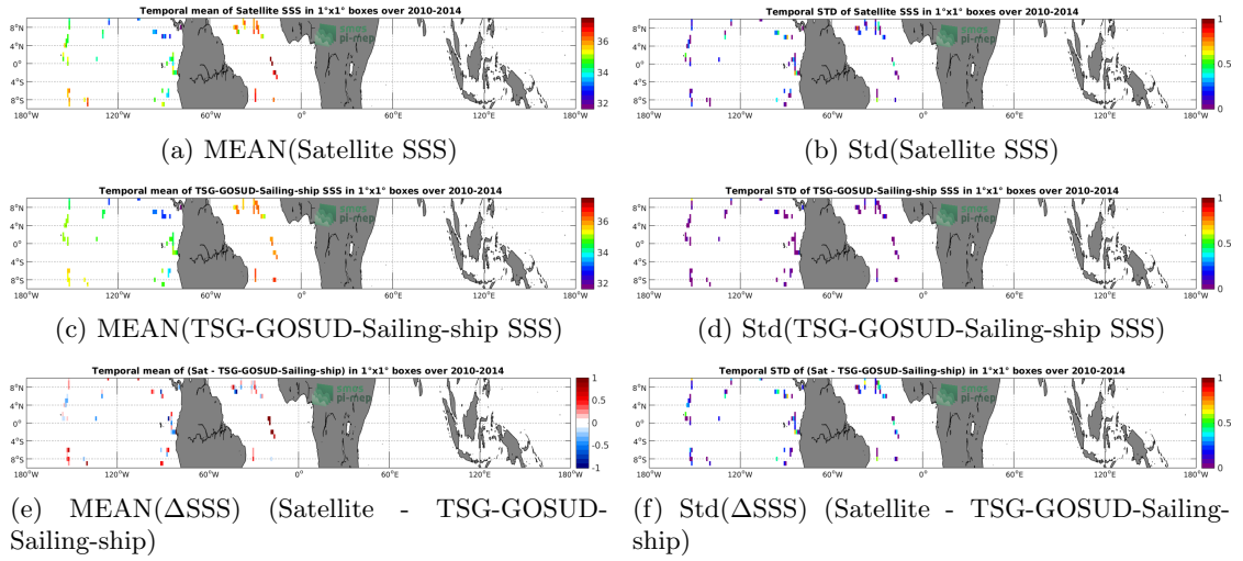
Figure 6: Temporal mean (left) and Std (right) of SSS from SMOS-L3-CATDS-CPDC-V321-L2Q (top), TSG-GOSUD-Sailing-ship (middle), and of \Delta SSS (Satellite - TSG-GOSUD-Sailing-ship). Only match-up pairs are used to generate these maps.
