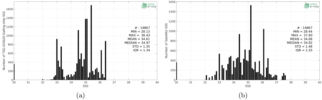
Figure 2: Histograms of SSS from TSG-GOSUD-Sailing-ship (a) and SMOS-L3-CATDS-CPDC-V321-L2Q (b) considering all match-up pairs per bins of 0.1 over the Equatorial Ocean 10N-10S Pi-MEP region and for the full satellite product period.
