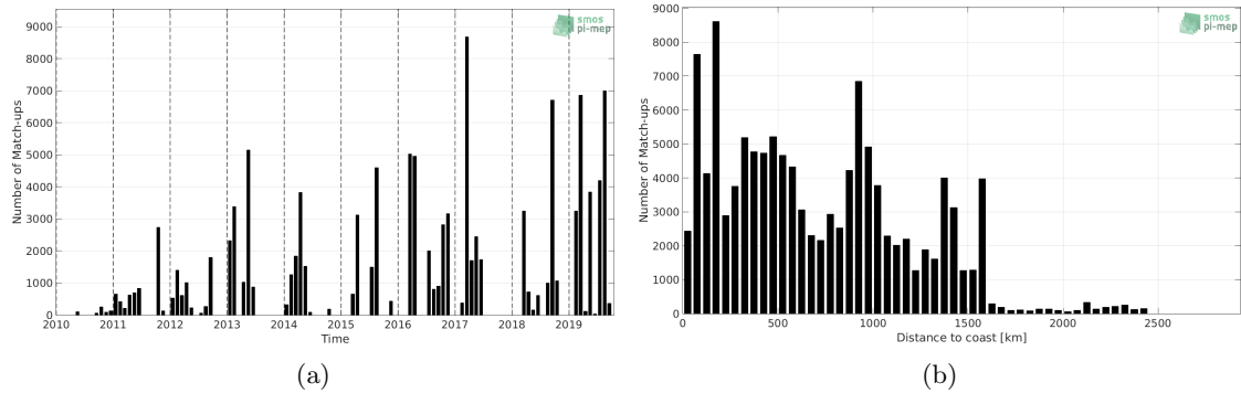
Figure 1: Number of match-ups between TSG (GOSUD-Research-vessel) and SMOS SSS L2Q v321 - 0.25 Deg (CATDS-CPDC) SSS as a function of time (a) and as function of the distance to coast (b) over the Equatorial Ocean 10N-10S Pi-MEP region and for the full satellite product period.
