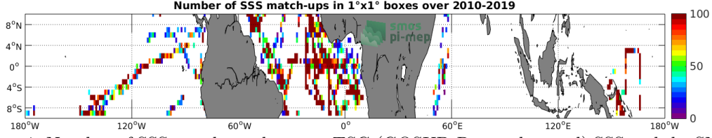
Figure 4: Number of SSS match-ups between TSG (GOSUD-Research-vessel) SSS and the SMOS SSS L2Q v321 - 0.25 Deg (CATDS-CPDC) SSS product for the Equatorial Ocean 10N-10S Pi-MEP region over 1^\circ \times 1^\circ boxes and for the full satellite product period.
