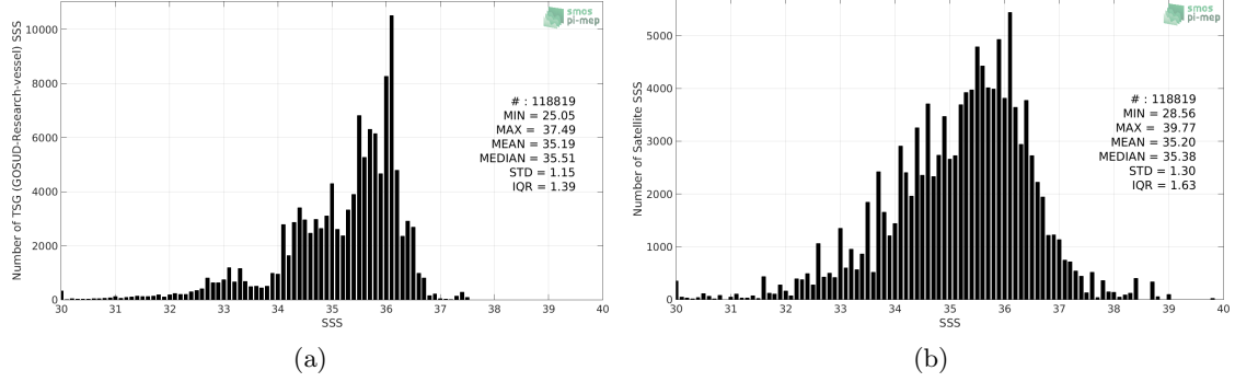
Figure 2: Histograms of SSS from TSG (GOSUD-Research-vessel) (a) and SMOS SSS L2Q v321 - 0.25 Deg (CATDS-CPDC) (b) considering all match-up pairs per bins of 0.1 over the Equatorial Ocean 10N-10S Pi-MEP region and for the full satellite product period.
