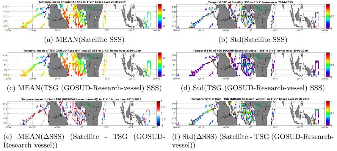
Figure 6: Temporal mean (left) and Std (right) of SSS from SMOS SSS L2Q v321 - 0.25 Deg (CATDS-CPDC) (top), TSG (GOSUD-Research-vessel) (middle), and of \Delta SSS (Satellite - TSG (GOSUD-Research-vessel)). Only match-up pairs are used to generate these maps.
