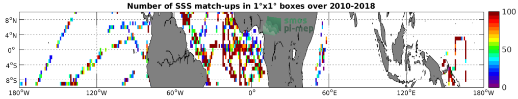
Figure 4: Number of SSS match-ups between TSG-GOSUD-Research-vessel SSS and the SMOS L2Q v321 - 0.25 Deg (CATDS-CPDC) SSS product for the Equatorial Ocean 10N-10S Pi-MEP region over 1°x1° boxes and for the full satellite product period.
