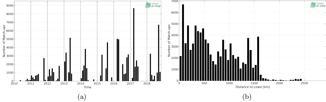
Figure 1: Number of match-ups between TSG-GOSUD-Research-vessel and SMOS L2Q v321 - 0.25 Deg (CATDS-CPDC) SSS as a function of time (a) and as function of the distance to coast (b) over the Equatorial Ocean 10N-10S Pi-MEP region and for the full satellite product period.
