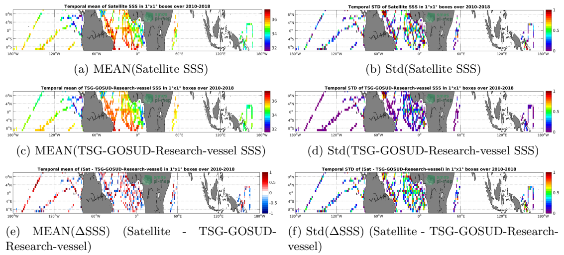
Figure 6: Temporal mean (left) and Std (right) of SSS from SMOS L2Q v321 - 0.25 Deg (CATDS-CPDC) (top), TSG-GOSUD-Research-vessel (middle), and of \Delta SSS (Satellite - TSG-GOSUD-Research-vessel). Only match-up pairs are used to generate these maps.
