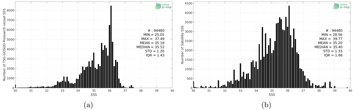
Figure 2: Histograms of SSS from TSG-GOSUD-Research-vessel (a) and SMOS L2Q v321 - 0.25 Deg (CATDS-CPDC) (b) considering all match-up pairs per bins of 0.1 over the Equatorial Ocean 10N-10S Pi-MEP region and for the full satellite product period.
