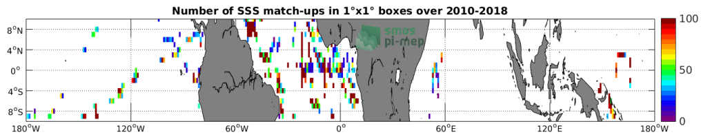
Figure 4: Number of SSS match-ups between TSG-GOSUD-Research-vessel SSS and the SMOS-L3-CATDS-CPDC-V321-L2Q SSS product for the Equatorial Ocean 10N-10S Pi-MEP region over 1°x1° boxes and for the full satellite product period.
