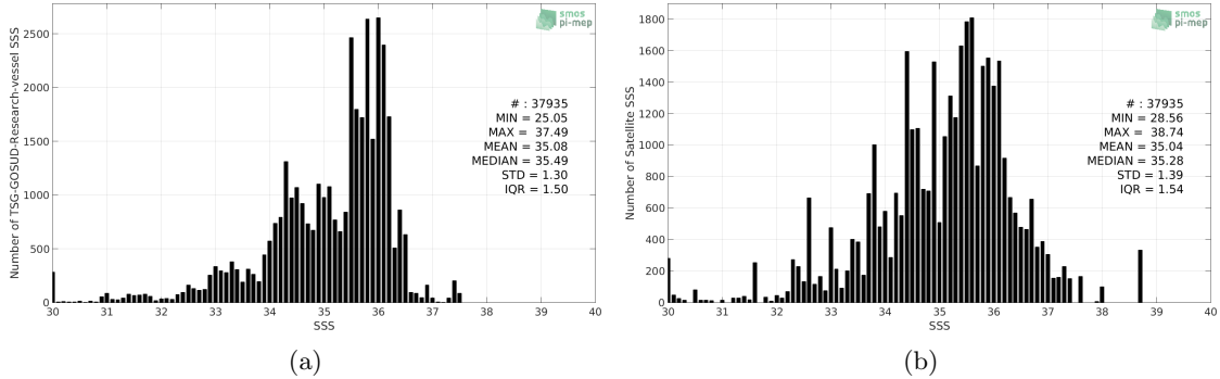
Figure 2: Histograms of SSS from TSG-GOSUD-Research-vessel (a) and SMOS-L3-CATDS-CPDC-V321-L2Q (b) considering all match-up pairs per bins of 0.1 over the Equatorial Ocean 10N-10S Pi-MEP region and for the full satellite product period.
