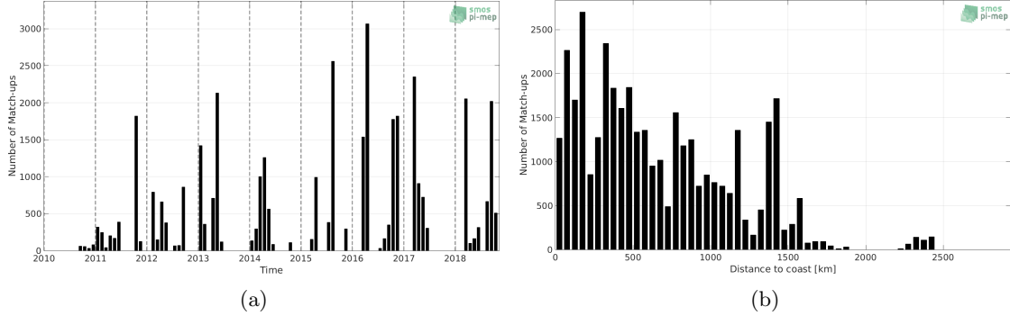
Figure 1: Number of match-ups between TSG-GOSUD-Research-vessel and SMOS-L3-CATDS-CPDC-V321-L2Q SSS as a function of time (a) and as function of the distance to coast (b) over the Equatorial Ocean 10N-10S Pi-MEP region and for the full satellite product period.
