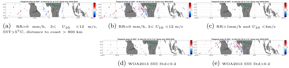
Figure 12: Temporal mean gridded over spatial boxes of size 1^\circ \times 1^\circ of \Delta SSS (SMOS-L3-CATDS-CPDC-V321-L2Q - TSG-GOSUD-Research-vessel) for 5 different subdatasets corresponding to: RR=0 mm/h, 3 < U_{10} < 12 m/s, SST>5°C, distance to coast > 800 km (a), RR=0 mm/h, 3 < U_{10} < 12 m/s (b), RR>1mm/h and U_{10} < 4 m/s (c), WOA2013 SSS Std<0.2 (d), WOA2013 SSS Std>0.2 (e).
