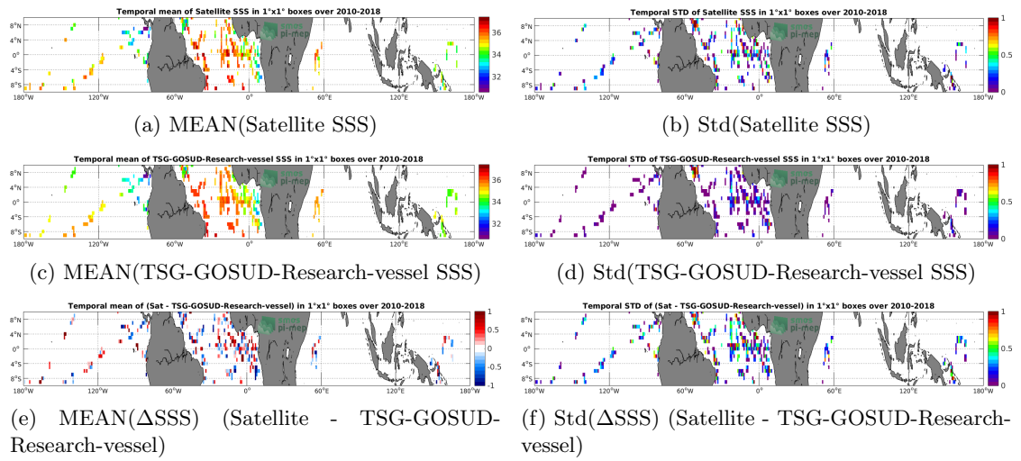
Figure 6: Temporal mean (left) and Std (right) of SSS from SMOS-L3-CATDS-CPDC-V321-L2Q (top), TSG-GOSUD-Research-vessel (middle), and of \Delta SSS (Satellite - TSG-GOSUD-Research-vessel). Only match-up pairs are used to generate these maps.
