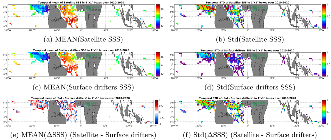
Figure 5: Temporal mean (left) and Std (right) of SSS from SMOS SSS L2Q v321 - 0.25 Deg (CATDS-CPDC) (top), Surface drifters (middle), and of \Delta SSS (Satellite - Surface drifters). Only match-up pairs are used to generate these maps.
