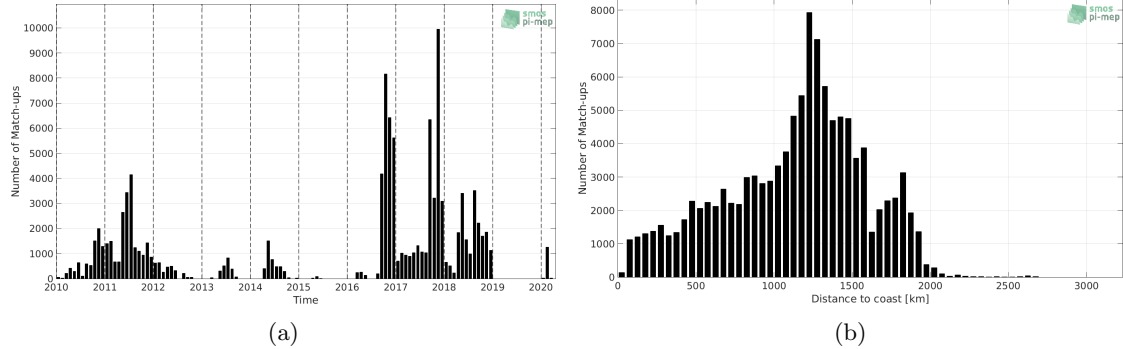
Figure 1: Number of match-ups between Surface drifters and SMOS SSS L2Q v321 - 0.25 Deg (CATDS-CPDC) SSS as a function of time (a) and as function of the distance to coast (b) over the Equatorial Ocean 10N-10S Pi-MEP region and for the full satellite product period.
