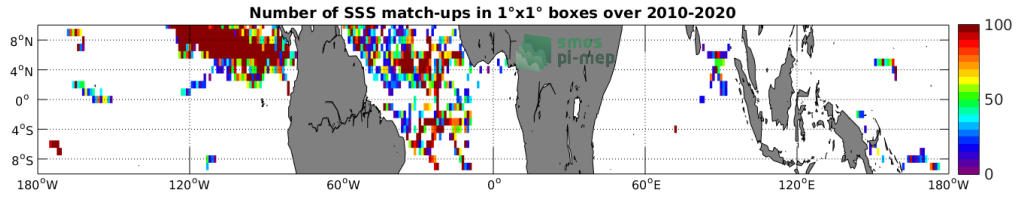
Figure 3: Number of SSS match-ups between Surface drifters SSS and the SMOS SSS L2Q v321 - 0.25 Deg (CATDS-CPDC) SSS product for the Equatorial Ocean 10N-10S Pi-MEP region over 1^\circ \times 1^\circ boxes and for the full satellite product period.
