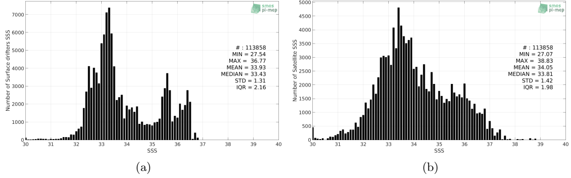
Figure 2: Histograms of SSS from Surface drifters (a) and SMOS SSS L2Q v321 - 0.25 Deg (CATDS-CPDC) (b) considering all match-up pairs per bins of 0.1 over the Equatorial Ocean 10N-10S Pi-MEP region and for the full satellite product period.
