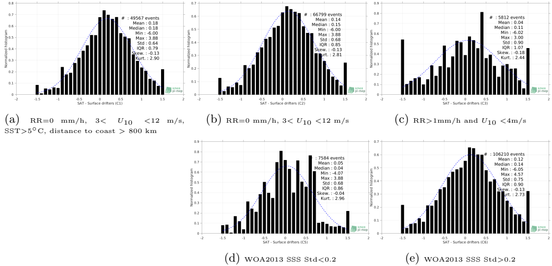
Figure 12: Normalized histogram of \Delta SSS (SMOS SSS L2Q v321 - 0.25 Deg (CATDS-CPDC) - Surface drifters) for 5 different subdatasets corresponding to: RR=0 mm/h, 3 < U_{10} < 12 m/s, SST >5^\circ\text{C} , distance to coast > 800 km (a), RR=0 mm/h, 3 < U_{10} < 12 m/s (b), RR >1 mm/h and U_{10} < 4 m/s (c), WOA2013 SSS Std <0.2 (d), WOA2013 SSS Std >0.2 (e).
