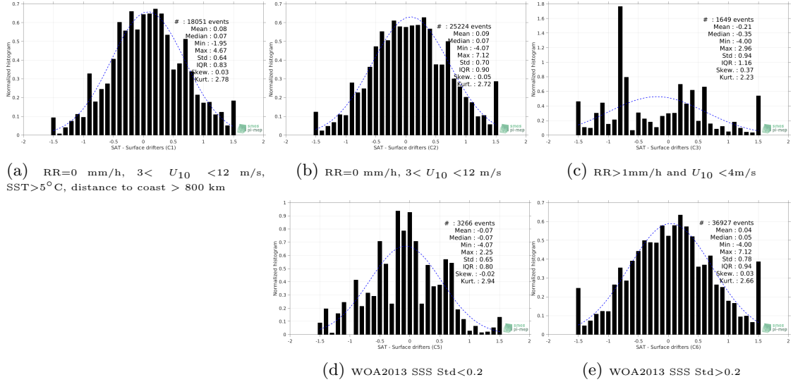
Figure 12: Normalized histogram of \Delta SSS (SMOS-L3-CATDS-CPDC-V321-L2Q - Surface drifters) for 5 different subsets corresponding to: RR=0 mm/h, 3 < U_{10} < 12 m/s, SST > 5^\circ C , distance to coast > 800 km (a), RR=0 mm/h, 3 < U_{10} < 12 m/s (b), RR > 1 mm/h and U_{10} < 4 m/s (c), WOA2013 SSS Std < 0.2 (d), WOA2013 SSS Std > 0.2 (e).
