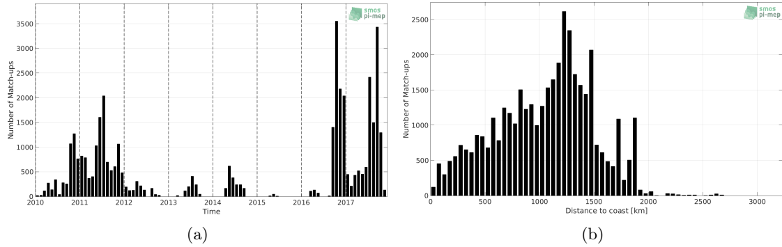
Figure 1: Number of match-ups between Surface drifters and SMOS-L3-CATDS-CPDC-V321-L2Q SSS as a function of time (a) and as function of the distance to coast (b) over the Equatorial Ocean 10N-10S Pi-MEP region and for the full satellite product period.
