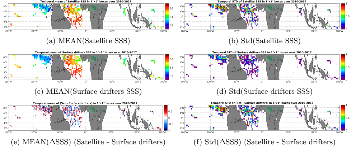
Figure 5: Temporal mean (left) and Std (right) of SSS from SMOS-L3-CATDS-CPDC-V321-L2Q (top), Surface drifters (middle), and of \Delta SSS (Satellite - Surface drifters). Only match-up pairs are used to generate these maps.
