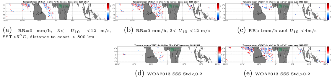
Figure 11: Temporal mean gridded over spatial boxes of size 1^\circ \times 1^\circ of \Delta SSS (SMOS-L3-CATDS-CPDC-V321-L2Q - Surface drifters) for 5 different subsets corresponding to: RR=0 mm/h, 3 < U_{10} < 12 m/s, SST > 5^\circ C , distance to coast > 800 km (a), RR=0 mm/h, 3 < U_{10} < 12 m/s (b), RR > 1 mm/h and U_{10} < 4 m/s (c), WOA2013 SSS Std < 0.2 (d), WOA2013 SSS Std > 0.2 (e).
