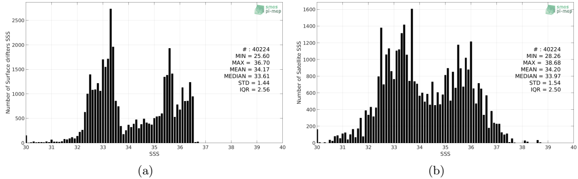
Figure 2: Histograms of SSS from Surface drifters (a) and SMOS-L3-CATDS-CPDC-V321-L2Q (b) considering all match-up pairs per bins of 0.1 over the Equatorial Ocean 10N-10S Pi-MEP region and for the full satellite product period.
