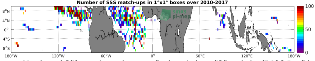
Figure 3: Number of SSS match-ups between Surface drifters SSS and the SMOS-L3-CATDS-CPDC-V321-L2Q SSS product for the Equatorial Ocean 10N-10S Pi-MEP region over 1^\circ \times 1^\circ boxes and for the full satellite product period.
