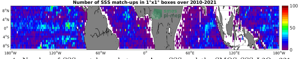
Figure 4: Number of SSS match-ups between Argo SSS and the SMOS SSS L2Q v321 - 0.25 Deg (CATDS-CPDC) SSS product for the Equatorial Ocean 10N-10S Pi-MEP region over 1^\circ \times 1^\circ boxes and for the full satellite product period.
