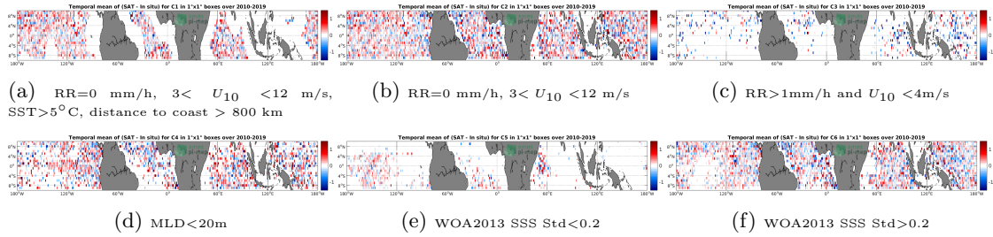
Figure 12: Temporal mean gridded over spatial boxes of size 1^\circ \times 1^\circ of \Delta SSS (SMOS-L3-CATDS-CPDC-V321-L2Q - Argo) for 6 different subdatasets corresponding to: RR=0 mm/h, 3 < U_{10} < 12 m/s, SST >5^\circ\text{C} , distance to coast > 800 km (a), RR=0 mm/h, 3 < U_{10} < 12 m/s (b), RR >1 mm/h and U_{10} < 4 m/s (c), MLD <20 m (d), WOA2013 SSS Std <0.2 (e), WOA2013 SSS Std >0.2 (f).
