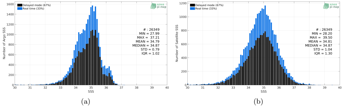
Figure 2: Histograms of SSS from Argo (a) and SMOS-L3-CATDS-CPDC-V321-L2Q (b) considering all match-up pairs per bins of 0.1 over the Equatorial Ocean 10N-10S Pi-MEP region and for the full satellite product period.
