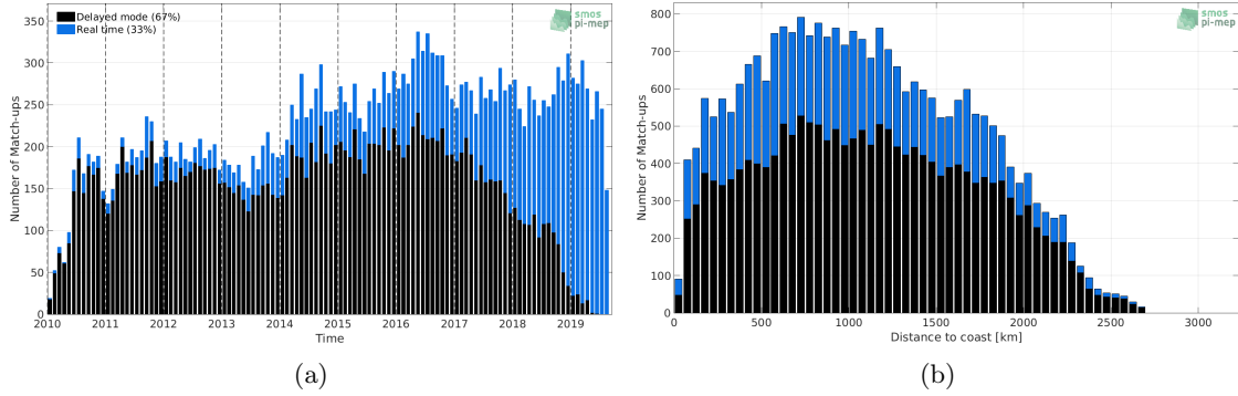
Figure 1: Number of match-ups between Argo and SMOS-L3-CATDS-CPDC-V321-L2Q SSS as a function of time (a) and as function of the distance to coast (b) over the Equatorial Ocean 10N-10S Pi-MEP region and for the full satellite product period.
