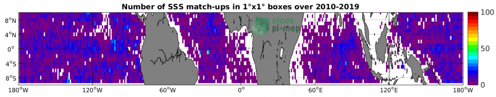
Figure 4: Number of SSS match-ups between Argo SSS and the SMOS-L3-CATDS-CPDC-V321-L2Q SSS product for the Equatorial Ocean 10N-10S Pi-MEP region over 1°x1° boxes and for the full satellite product period.
