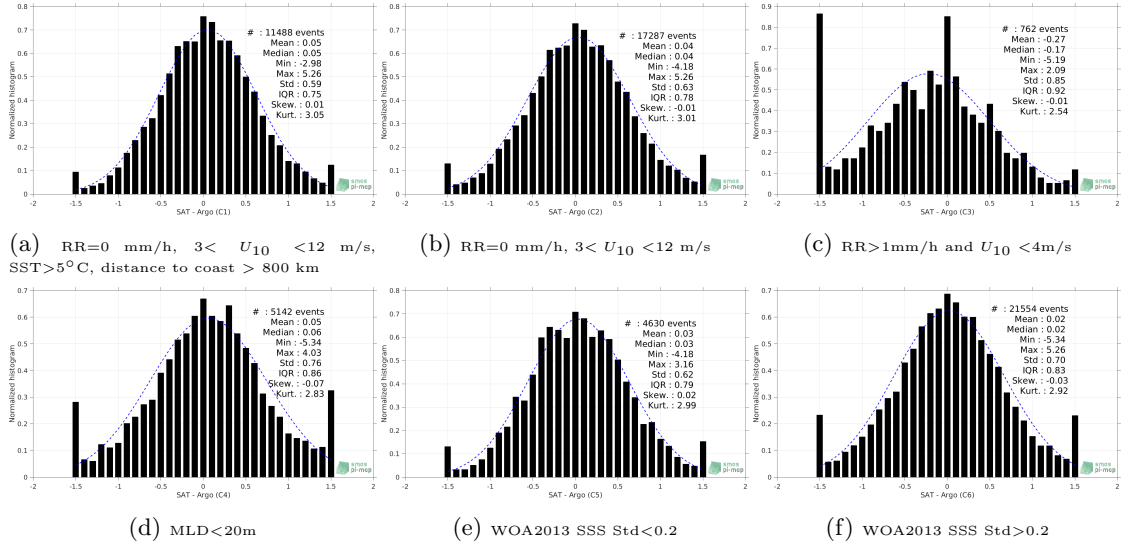
Figure 13: Normalized histogram of \Delta SSS (SMOS-L3-CATDS-CPDC-V321-L2Q - Argo) for 6 different subdatasets corresponding to: RR=0 mm/h, 3 < U_{10} < 12 m/s, SST >5^\circ\text{C} , distance to coast > 800 km (a), RR=0 mm/h, 3 < U_{10} < 12 m/s (b), RR >1 mm/h and U_{10} < 4 m/s (c), MLD <20 m (d), WOA2013 SSS Std <0.2 (e), WOA2013 SSS Std >0.2 (f).
