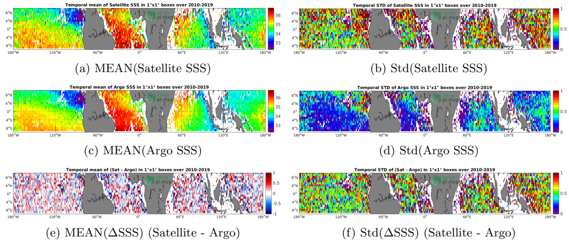
Figure 6: Temporal mean (left) and Std (right) of SSS from SMOS-L3-CATDS-CPDC-V321-L2Q (top), Argo (middle), and of \Delta SSS (Satellite - Argo). Only match-up pairs are used to generate these maps.
