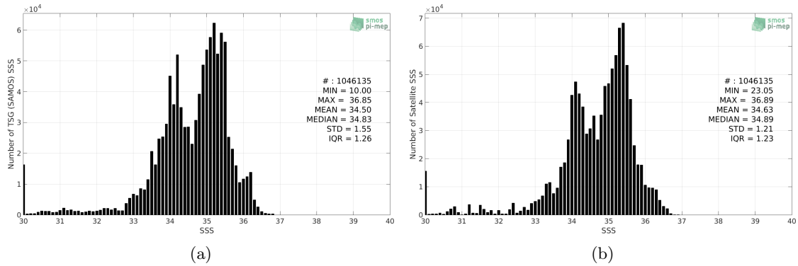
Figure 2: Histograms of SSS from TSG (SAMOS) (a) and SMOS SSS L3 v317 - Monthly - 25 km (CATDS-CPDC) (b) considering all match-up pairs per bins of 0.1 over the Equatorial Ocean 10N-10S Pi-MEP region and for the full satellite product period.
