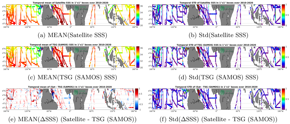
Figure 6: Temporal mean (left) and Std (right) of SSS from SMOS SSS L3 v317 - Monthly - 25 km (CATDS-CPDC) (top), TSG (SAMOS) (middle), and of \Delta SSS (Satellite - TSG (SAMOS)). Only match-up pairs are used to generate these maps.
