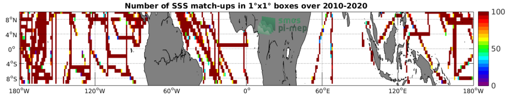
Figure 4: Number of SSS match-ups between TSG (SAMOS) SSS and the SMOS SSS L3 v317 - Monthly - 25 km (CATDS-CPDC) SSS product for the Equatorial Ocean 10N-10S Pi-MEP region over 1^\circ \times 1^\circ boxes and for the full satellite product period.
