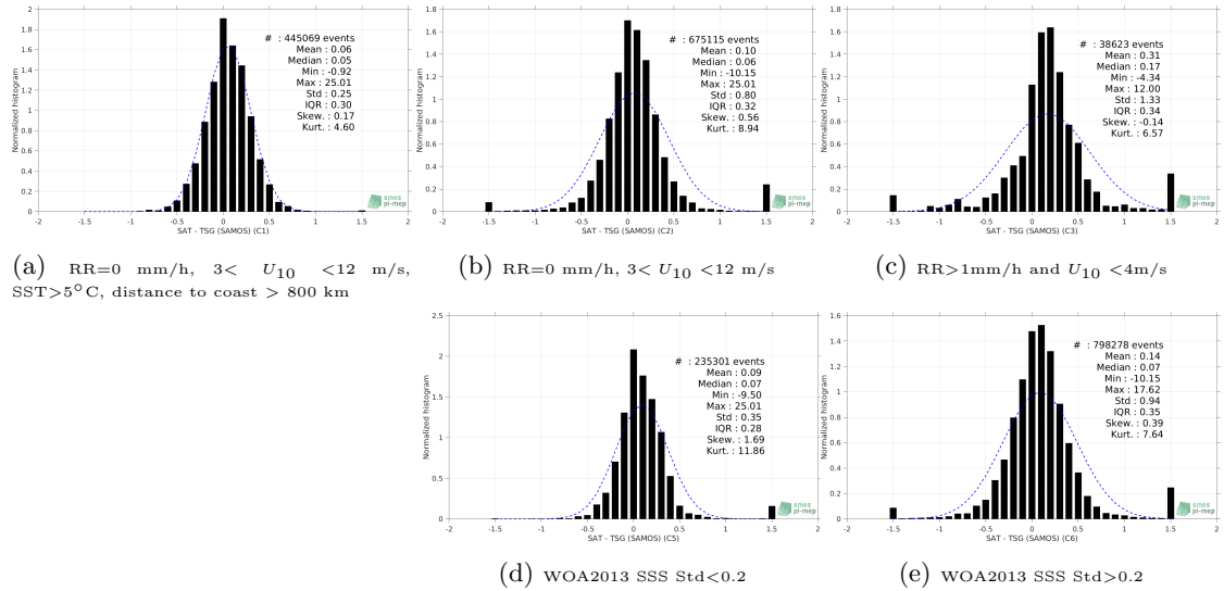
Figure 13: Normalized histogram of \Delta SSS (SMOS SSS L3 v317 - Monthly - 25 km (CATDS-CPDC) - TSG (SAMOS)) for 5 different subdatasets corresponding to: RR=0 mm/h, 3 < U_{10} < 12 m/s, SST > 5^\circ C , distance to coast > 800 km (a), RR=0 mm/h, 3 < U_{10} < 12 m/s (b), RR > 1 mm/h and U_{10} < 4 m/s (c), WOA2013 SSS Std < 0.2 (d), WOA2013 SSS Std > 0.2 (e).
