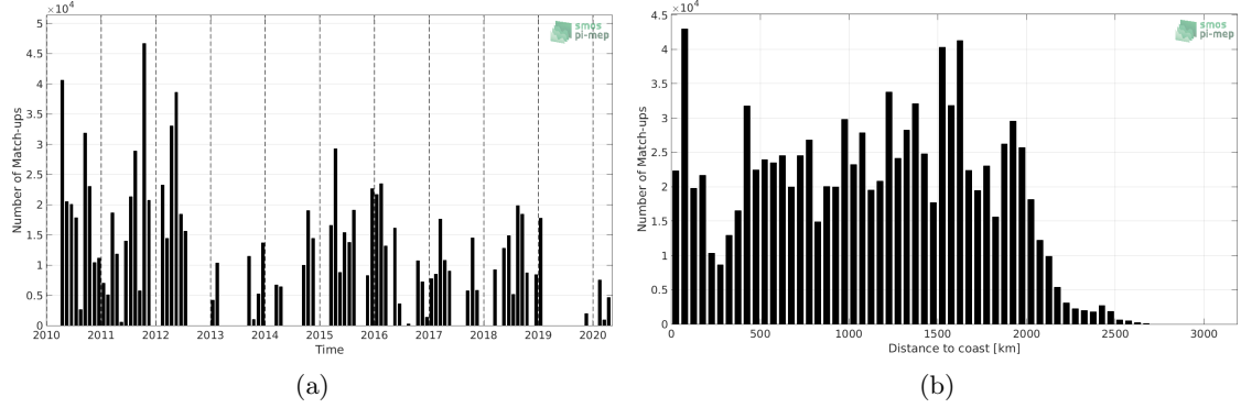
Figure 1: Number of match-ups between TSG (SAMOS) and SMOS SSS L3 v317 - Monthly - 25 km (CATDS-CPDC) SSS as a function of time (a) and as function of the distance to coast (b) over the Equatorial Ocean 10N-10S Pi-MEP region and for the full satellite product period.
