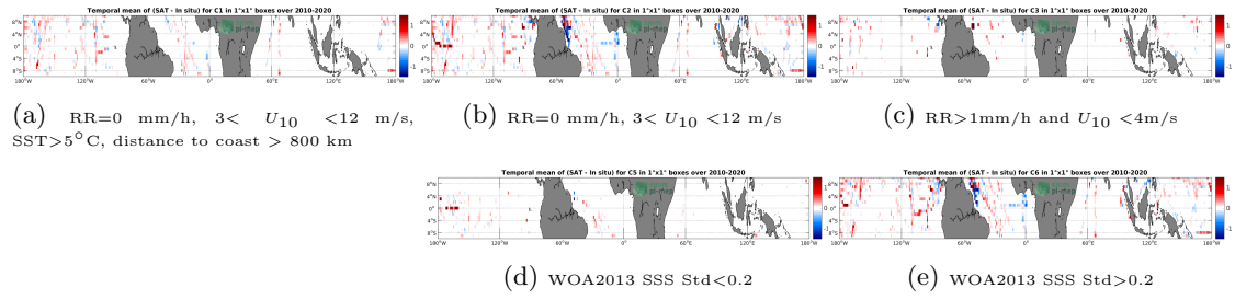
Figure 12: Temporal mean gridded over spatial boxes of size 1^\circ \times 1^\circ of \Delta SSS (SMOS SSS L3 v317 - Monthly - 25 km (CATDS-CPDC) - TSG (SAMOS)) for 5 different subdatasets corresponding to: RR=0 mm/h, 3 < U_{10} < 12 m/s, SST > 5^\circ C , distance to coast > 800 km (a), RR=0 mm/h, 3 < U_{10} < 12 m/s (b), RR > 1 mm/h and U_{10} < 4 m/s (c), WOA2013 SSS Std < 0.2 (d), WOA2013 SSS Std > 0.2 (e).
