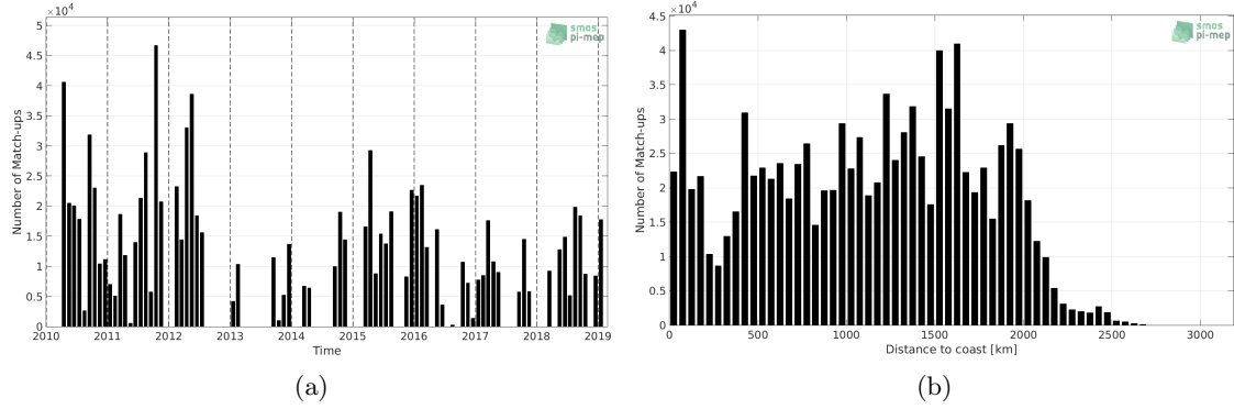
Figure 1: Number of match-ups between TSG-SAMOS and SMOS-L3-CATDS-CPDC-V317-MONTHLY-25KM SSS as a function of time (a) and as function of the distance to coast (b) over the Equatorial Ocean 10N-10S Pi-MEP region and for the full satellite product period.
