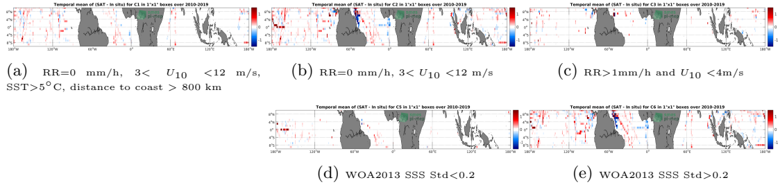
Figure 12: Temporal mean gridded over spatial boxes of size 1^\circ \times 1^\circ of \Delta SSS (SMOS-L3-CATDS-CPDC-V317-MONTHLY-25KM - TSG-SAMOS) for 5 different subdatasets corresponding to: RR=0 mm/h, 3 < U_{10} < 12 m/s, SST > 5^\circ C , distance to coast > 800 km (a), RR=0 mm/h, 3 < U_{10} < 12 m/s (b), RR > 1 mm/h and U_{10} < 4 m/s (c), WOA2013 SSS Std < 0.2 (d), WOA2013 SSS Std > 0.2 (e).
