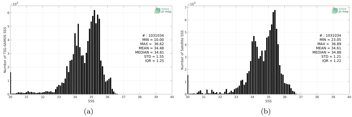
Figure 2: Histograms of SSS from TSG-SAMOS (a) and SMOS-L3-CATDS-CPDC-V317-MONTHLY-25KM (b) considering all match-up pairs per bins of 0.1 over the Equatorial Ocean 10N-10S Pi-MEP region and for the full satellite product period.
