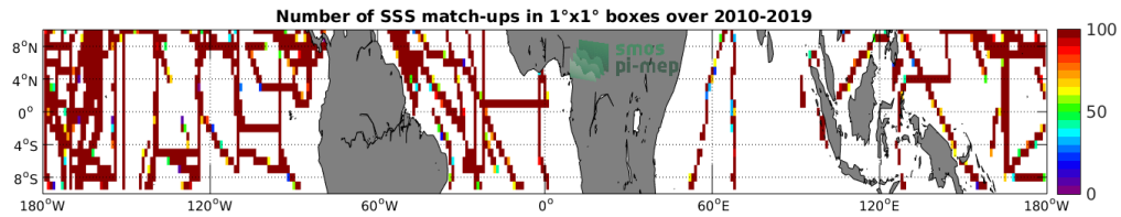
Figure 4: Number of SSS match-ups between TSG-SAMOS SSS and the SMOS-L3-CATDS-CPDC-V317-MONTHLY-25KM SSS product for the Equatorial Ocean 10N-10S Pi-MEP region over 1^\circ \times 1^\circ boxes and for the full satellite product period.
