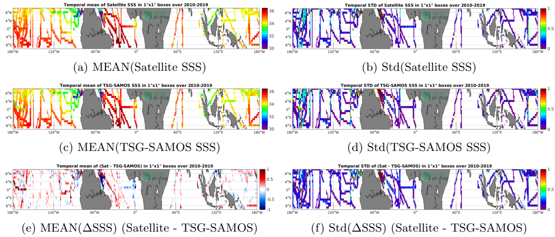
Figure 6: Temporal mean (left) and Std (right) of SSS from SMOS-L3-CATDS-CPDC-V317-MONTHLY-25KM (top), TSG-SAMOS (middle), and of \Delta SSS (Satellite - TSG-SAMOS). Only match-up pairs are used to generate these maps.
