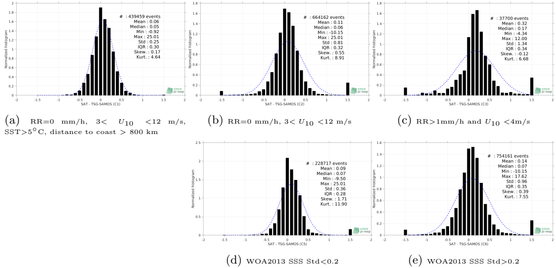
Figure 13: Normalized histogram of \Delta SSS (SMOS-L3-CATDS-CPDC-V317-MONTHLY-25KM - TSG-SAMOS) for 5 different subdatasets corresponding to: RR=0 mm/h, 3 < U_{10} < 12 m/s, SST > 5^\circ C , distance to coast > 800 km (a), RR=0 mm/h, 3 < U_{10} < 12 m/s (b), RR > 1 mm/h and U_{10} < 4 m/s (c), WOA2013 SSS Std < 0.2 (d), WOA2013 SSS Std > 0.2 (e).
