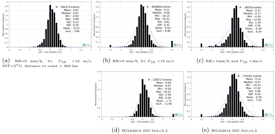
Figure 13: Normalized histogram of \Delta SSS (SMOS-L3-CATDS-CPDC-V317-MONTHLY-25KM - TSG-SAMOS) for 5 different subdatasets corresponding to: RR=0 mm/h, 3 < U_{10} < 12 m/s, SST >5^\circ C, distance to coast > 800 km (a), RR=0 mm/h, 3 < U_{10} < 12 m/s (b), RR >1 mm/h and U_{10} < 4 m/s (c), WOA2013 SSS Std <0.2 (d), WOA2013 SSS Std >0.2 (e).
