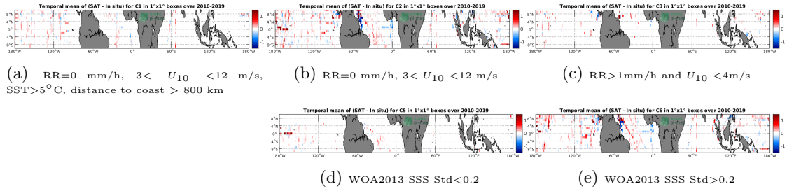
Figure 12: Temporal mean gridded over spatial boxes of size 1^\circ \times 1^\circ of \Delta SSS (SMOS-L3-CATDS-CPDC-V317-MONTHLY-25KM - TSG-SAMOS) for 5 different subdatasets corresponding to: RR=0 mm/h, 3 < U_{10} < 12 m/s, SST >5^\circ C, distance to coast > 800 km (a), RR=0 mm/h, 3 < U_{10} < 12 m/s (b), RR >1 mm/h and U_{10} < 4 m/s (c), WOA2013 SSS Std <0.2 (d), WOA2013 SSS Std >0.2 (e).
