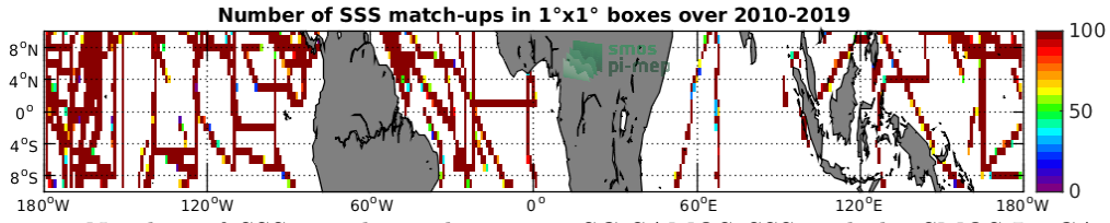
Figure 4: Number of SSS match-ups between TSG-SAMOS SSS and the SMOS-L3-CATDS-CPDC-V317-MONTHLY-25KM SSS product for the Equatorial Ocean 10N-10S Pi-MEP region over 1^\circ \times 1^\circ boxes and for the full satellite product period.
