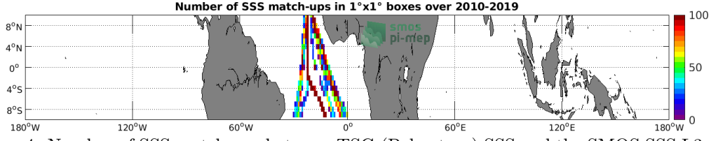
Figure 4: Number of SSS match-ups between TSG (Polarstern) SSS and the SMOS SSS L3 v317 - Monthly - 25 km (CATDS-CPDC) SSS product for the Equatorial Ocean 10N-10S Pi-MEP region over 1^\circ \times 1^\circ boxes and for the full satellite product period.
