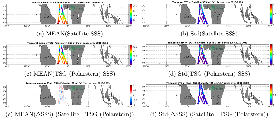
Figure 6: Temporal mean (left) and Std (right) of SSS from SMOS SSS L3 v317 - Monthly - 25 km (CATDS-CPDC) (top), TSG (Polarstern) (middle), and of \Delta SSS (Satellite - TSG (Polarstern)). Only match-up pairs are used to generate these maps.
