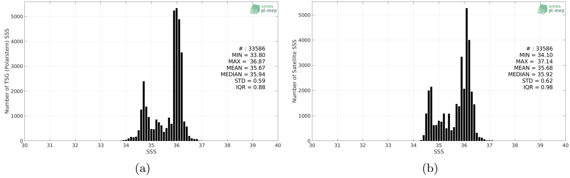
Figure 2: Histograms of SSS from TSG (Polarstern) (a) and SMOS SSS L3 v317 - Monthly - 25 km (CATDS-CPDC) (b) considering all match-up pairs per bins of 0.1 over the Equatorial Ocean 10N-10S Pi-MEP region and for the full satellite product period.
