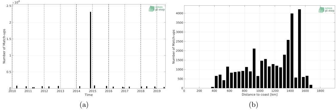
Figure 1: Number of match-ups between TSG (Polarstern) and SMOS SSS L3 v317 - Monthly - 25 km (CATDS-CPDC) SSS as a function of time (a) and as function of the distance to coast (b) over the Equatorial Ocean 10N-10S Pi-MEP region and for the full satellite product period.
