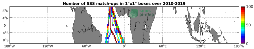
Figure 4: Number of SSS match-ups between TSG (Polarstern) SSS and the SMOS SSS L3 v317 - Monthly - 25 km (CATDS-CPDC) SSS product for the Equatorial Ocean 10N-10S Pi-MEP region over 1^\circ \times 1^\circ boxes and for the full satellite product period.
