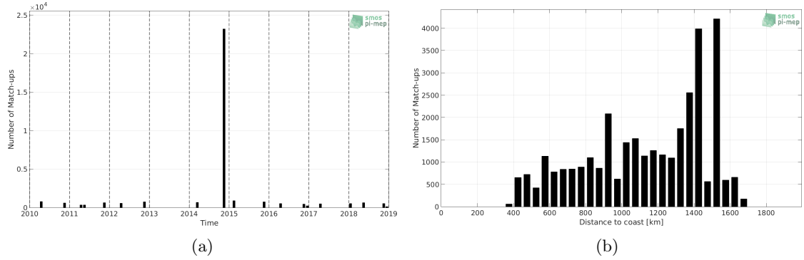
Figure 1: Number of match-ups between TSG (Polarstern) and SMOS SSS L3 v317 - Monthly - 25 km (CATDS-CPDC) SSS as a function of time (a) and as function of the distance to coast (b) over the Equatorial Ocean 10N-10S Pi-MEP region and for the full satellite product period.
