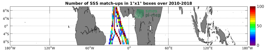
Figure 4: Number of SSS match-ups between TSG (Polarstern) SSS and the SMOS SSS L3 v317 - Monthly - 25 km (CATDS-CPDC) SSS product for the Equatorial Ocean 10N-10S Pi-MEP region over 1°x1° boxes and for the full satellite product period.
