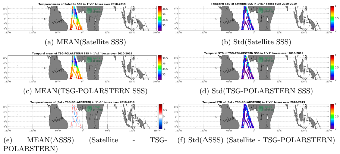
Figure 6: Temporal mean (left) and Std (right) of SSS from SMOS L3 v317 - Monthly - 25 km (CATDS-CPDC) (top), TSG-POLARSTERN (middle), and of \Delta SSS (Satellite - TSG-POLARSTERN). Only match-up pairs are used to generate these maps.
