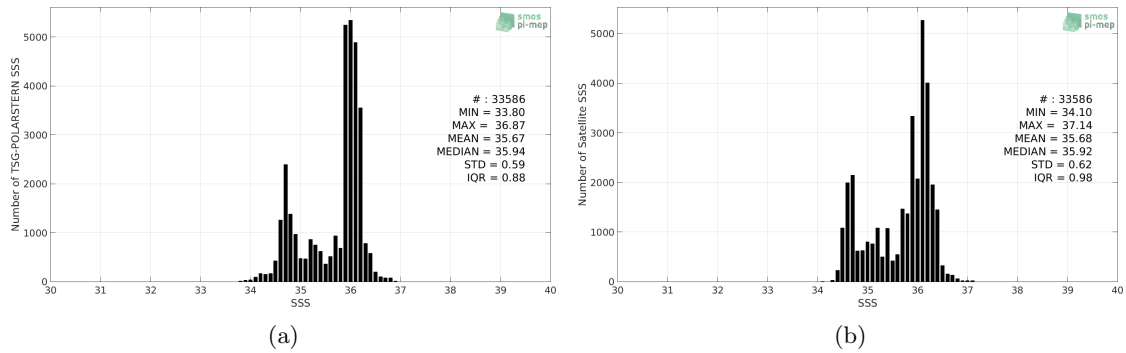
Figure 2: Histograms of SSS from TSG-POLARSTERN (a) and SMOS L3 v317 - Monthly - 25 km (CATDS-CPDC) (b) considering all match-up pairs per bins of 0.1 over the Equatorial Ocean 10N-10S Pi-MEP region and for the full satellite product period.
