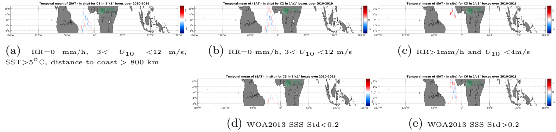
Figure 12: Temporal mean gridded over spatial boxes of size 1^{\circ}\times 1^{\circ} of \Delta\text{SSS} (SMOS L3 v317 - Monthly - 25 km (CATDS-CPDC) - TSG-POLARSTERN) for 5 different subdatasets corresponding to:RR=0 mm/h, 3 < U_{10} < 12 m/s, SST >5^{\circ}\text{C} , distance to coast > 800 km (a), RR=0 mm/h, 3 < U_{10} < 12 m/s (b), RR >1 mm/h and U_{10} < 4 m/s (c), WOA2013 SSS Std <0.2 (d), WOA2013 SSS Std >0.2 (e).
