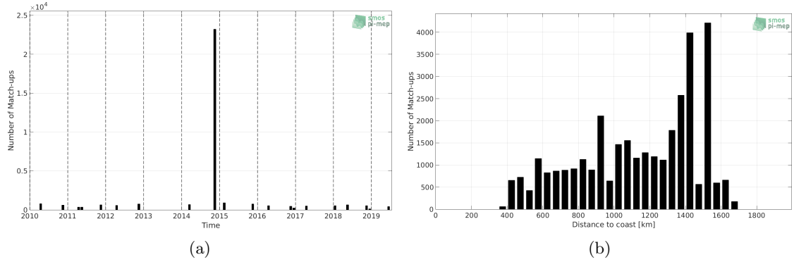
Figure 1: Number of match-ups between TSG-POLARSTERN and SMOS L3 v317 - Monthly - 25 km (CATDS-CPDC) SSS as a function of time (a) and as function of the distance to coast (b) over the Equatorial Ocean 10N-10S Pi-MEP region and for the full satellite product period.
