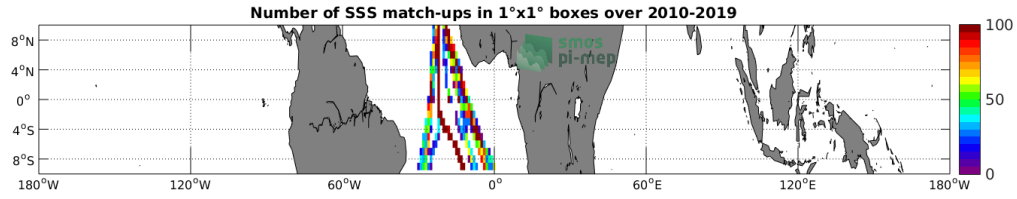
Figure 4: Number of SSS match-ups between TSG-POLARSTERN SSS and the SMOS L3 v317 - Monthly - 25 km (CATDS-CPDC) SSS product for the Equatorial Ocean 10N-10S Pi-MEP region over 1^\circ \times 1^\circ boxes and for the full satellite product period.
